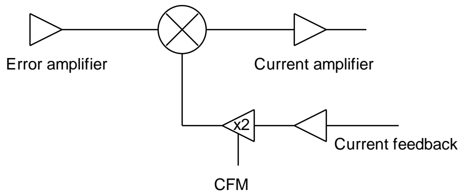
CFM BLOCK DIAGRAM
