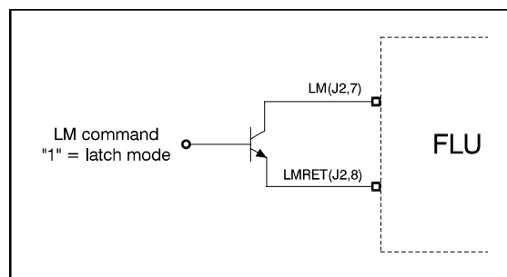
Figure 4-2: LM Remote Control
