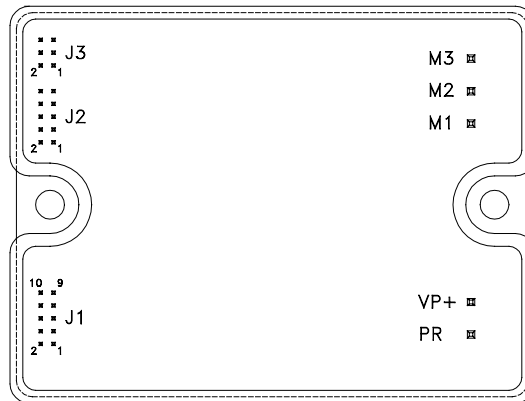
Figure 3-3: Flute Connector Locations
