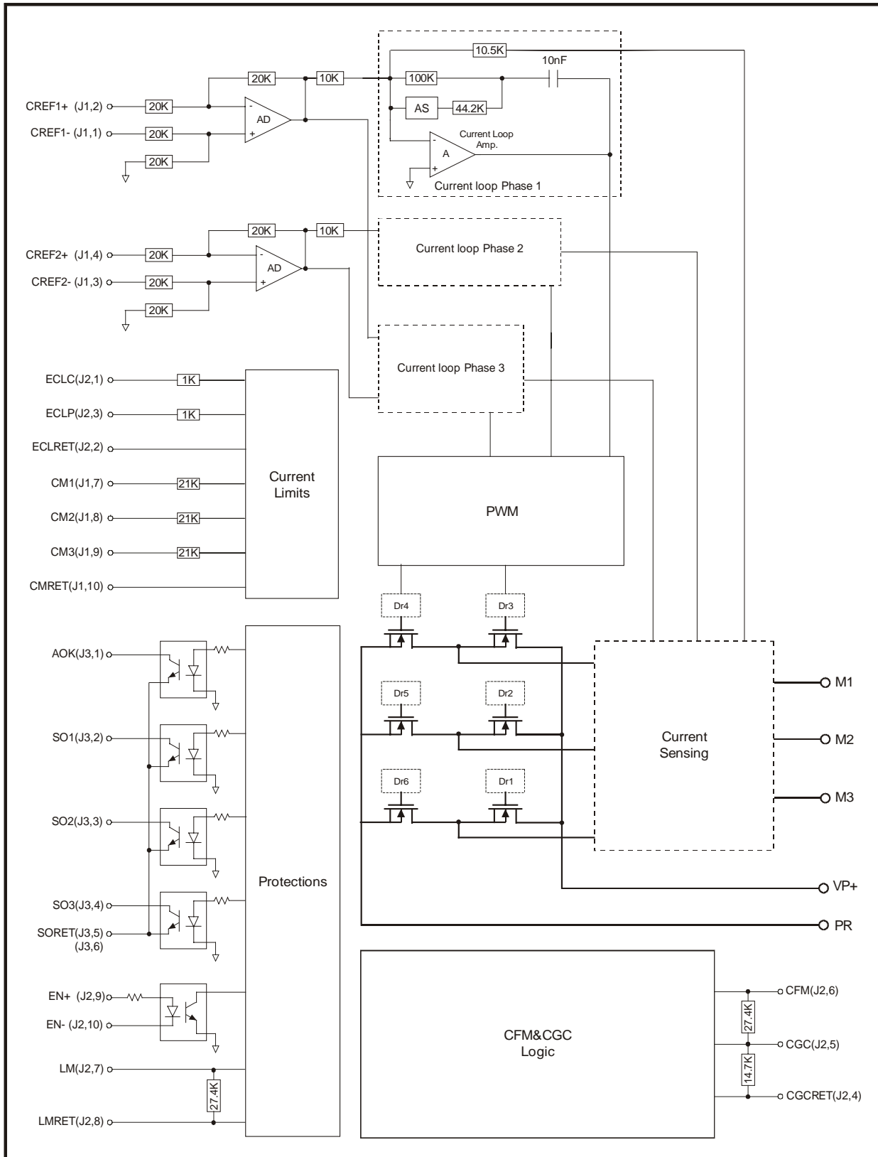
Figure 2-1: Flute Block Diagram
