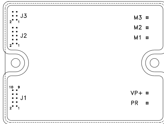
Figure 3-3: Raven Connector Locations
