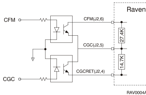
Figure 4-1: CFM and CGC Remote Control
