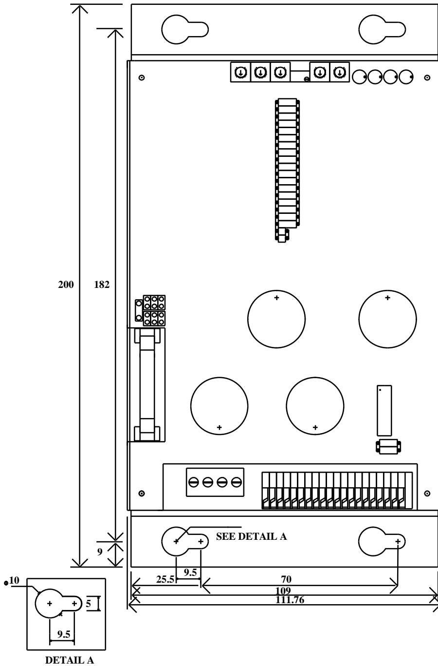
SP4 - TOP VIEW
