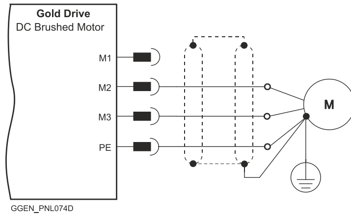
Figure 11: DC Brushed Motor Power Connection Diagram
