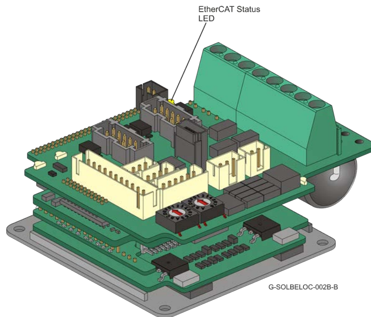
Figure 38: EtherCAT Status LED
