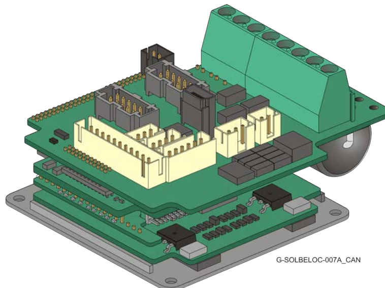
Figure 39: Gold Solo Bell (2 mm pitch E/C Conn.) - CAN
