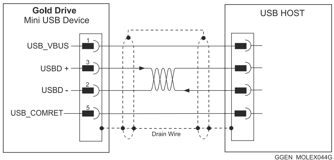
Figure 35: USB Network Diagram
