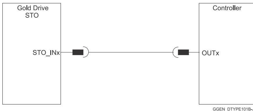
Figure 9: STO Cable Assemblies
