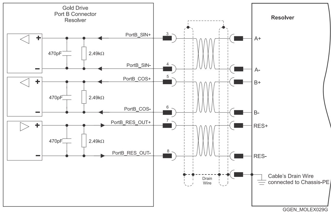
Figure 26: Port B – Resolver Shrouded Type Connection Diagram
