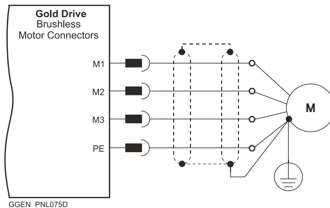
Figure 10: Brushless Motor Power Connection Diagram
