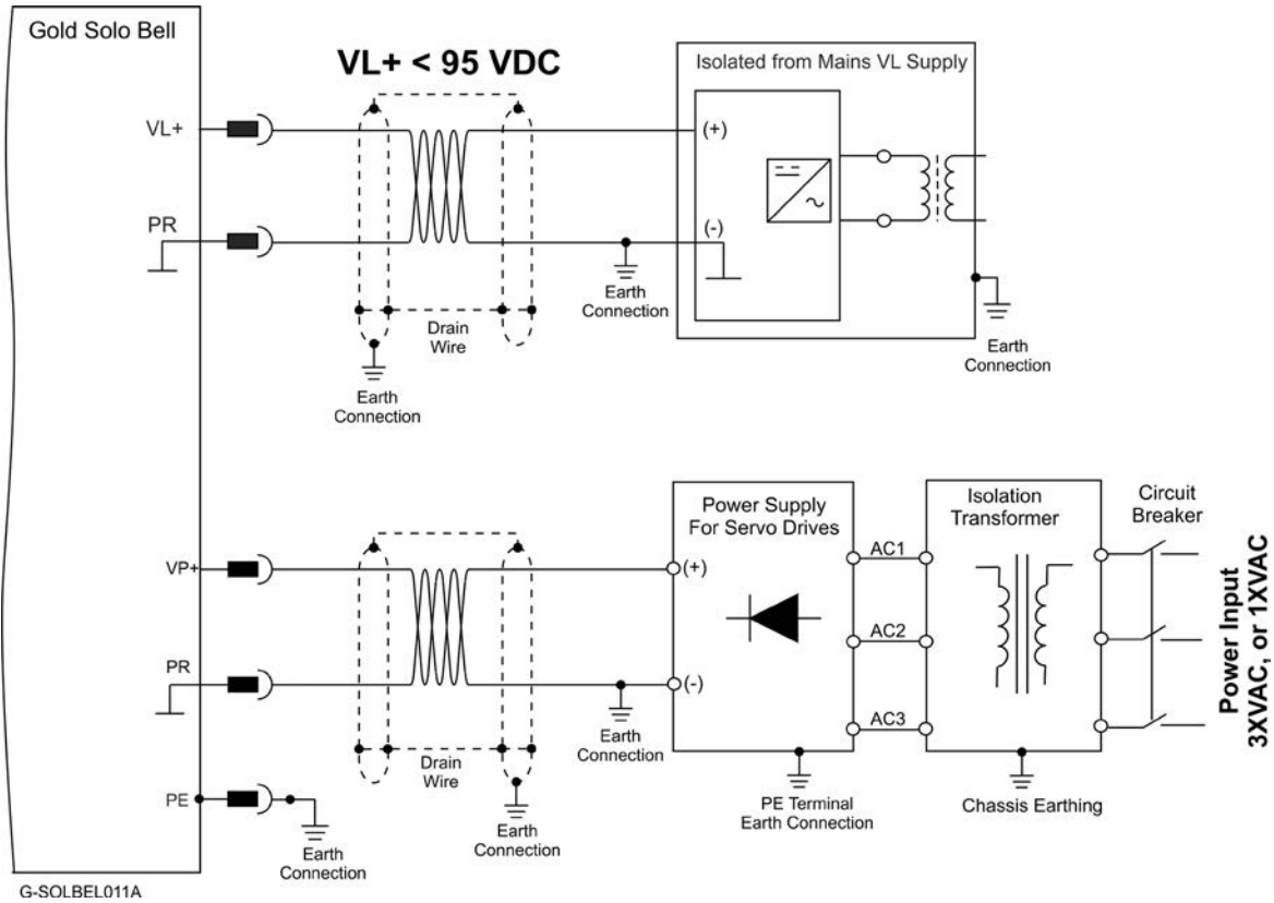
Figure 13: 200 VDC Power Source Connection Diagram
