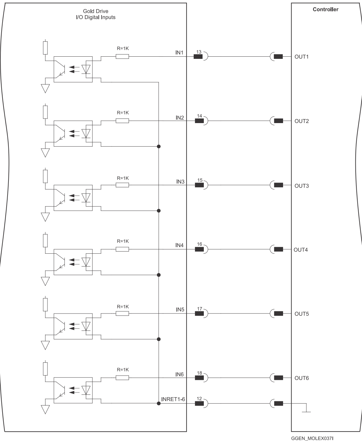
Figure 29: Digital Input TTL Mode Connection Diagram
