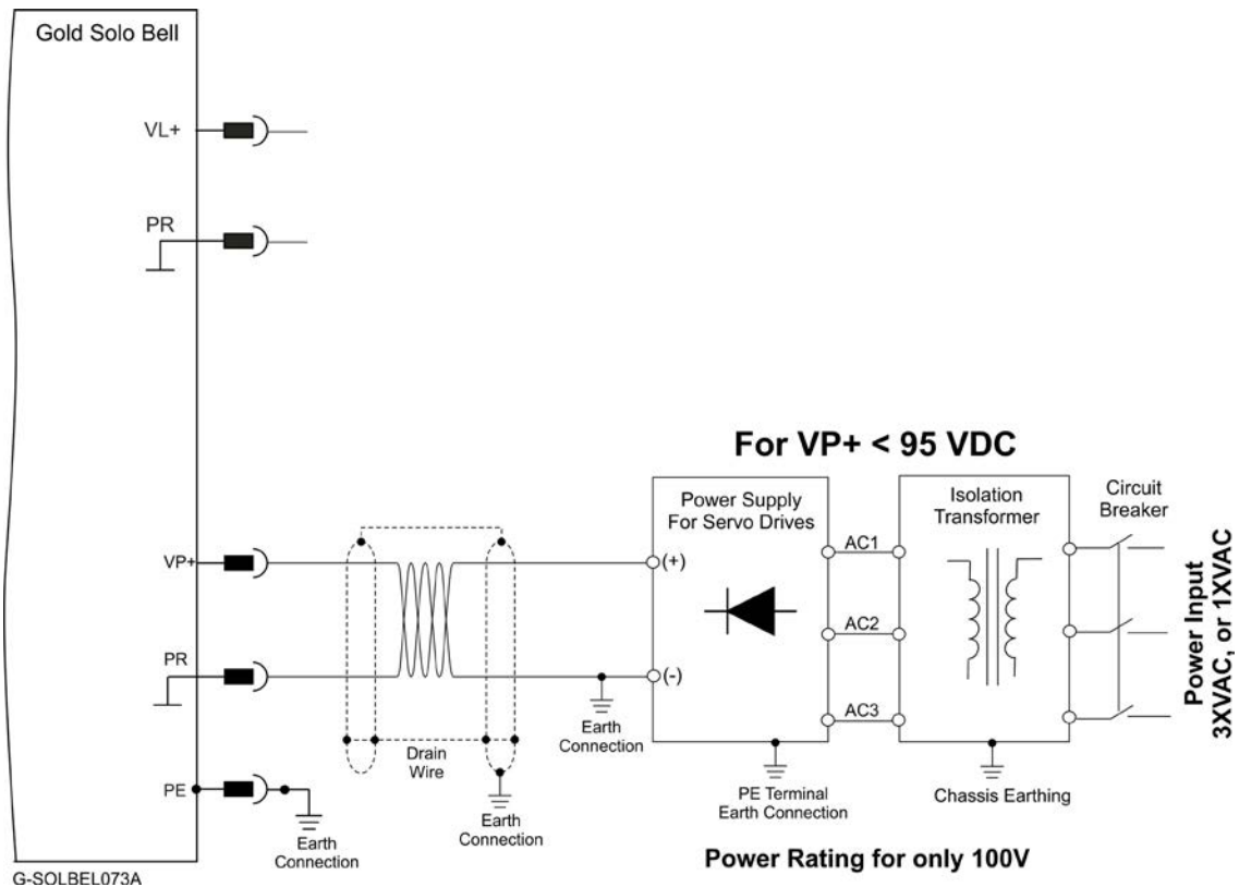
Figure 14: Main Power Supply Connection Diagram (No Control Supply)
