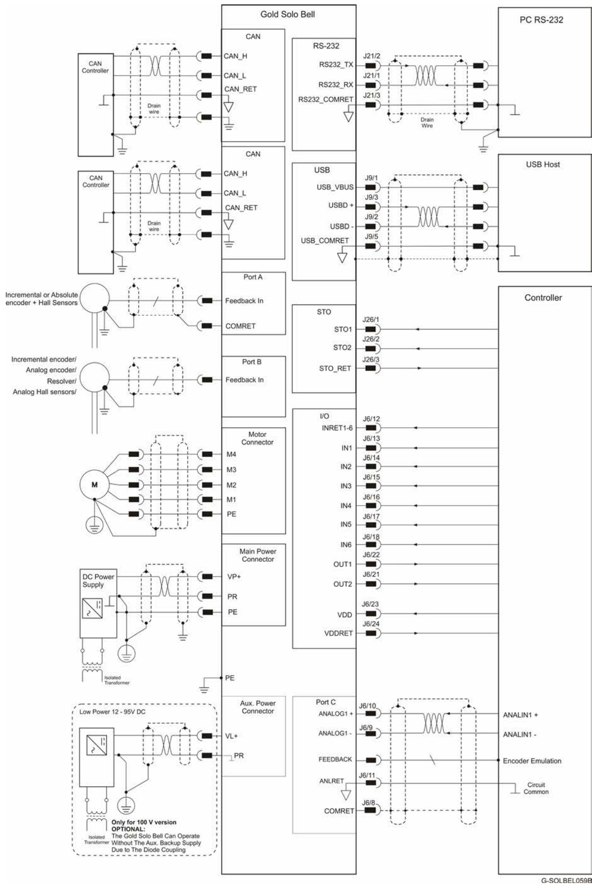
Figure 4: The Gold Solo Bell (2 mm pitch E/C Conn.) Connection Diagram – CAN
