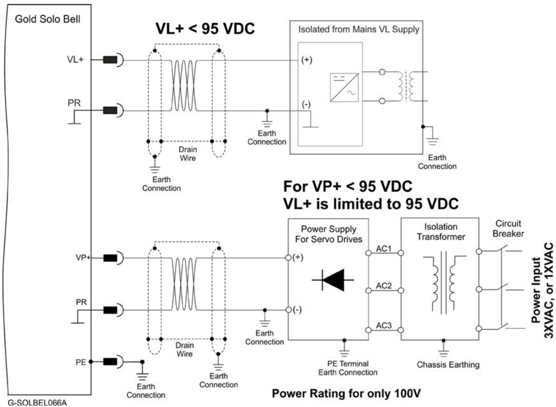
Figure 15: Control Supply Connection Diagram
