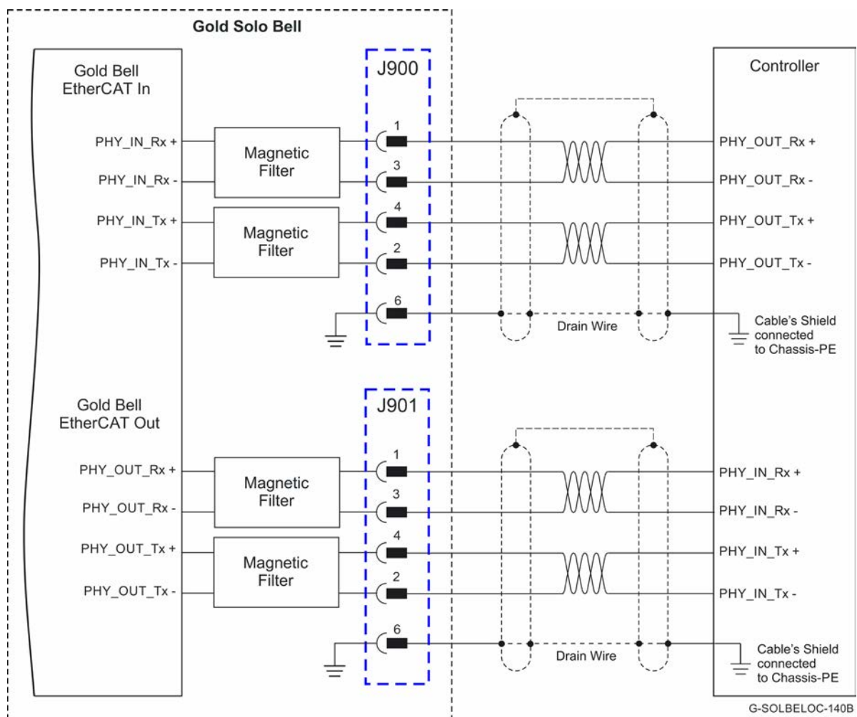
Figure 37: EtherCAT Connection Schematic Diagram
