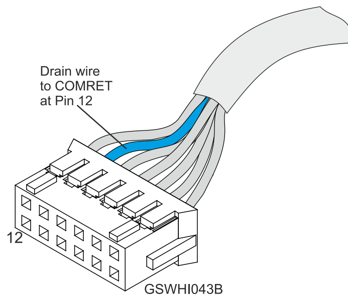
Figure 5: Feedback and Shrouded Control Cable Assemblies – Example
