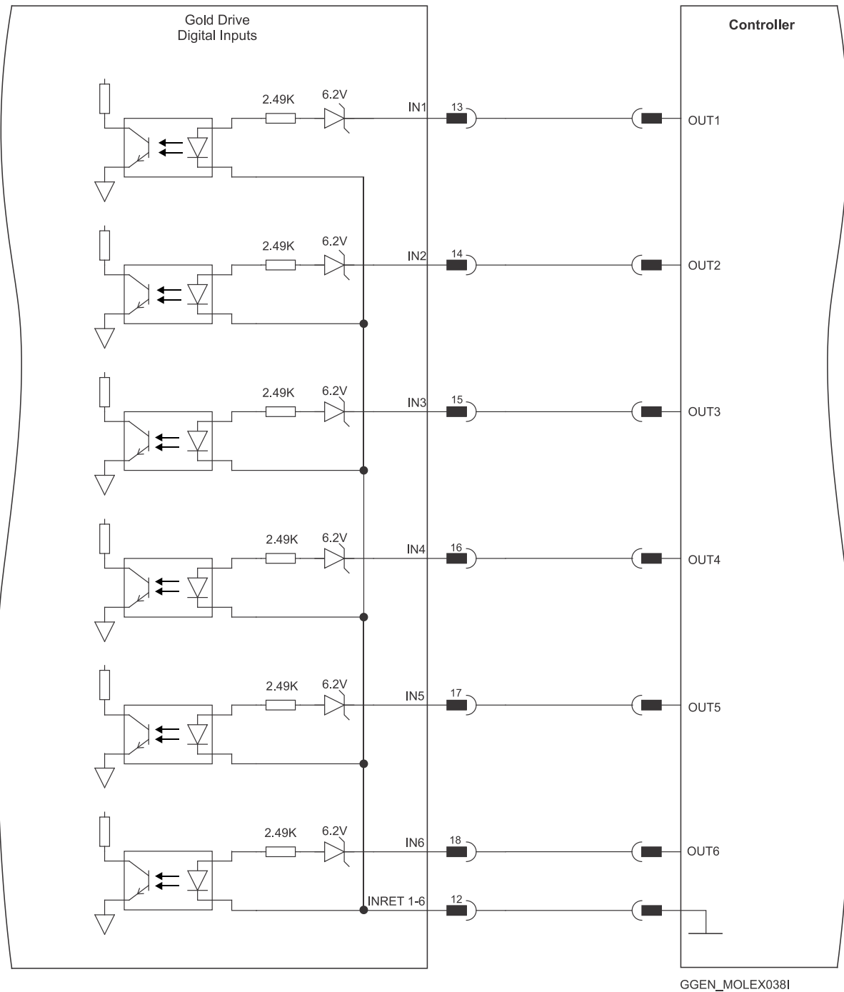
Figure 31: Digital Input Connection Diagram – Source PLC Option
