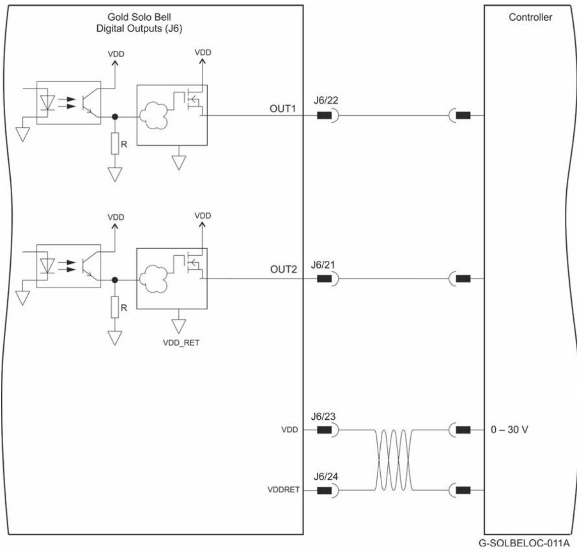
Figure 32: Digital Output Connection Diagram – Source PLC Option
