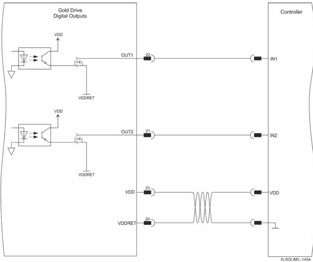
Figure 34: Digital Output as Sink Configuration Molex Type Connection Diagram
