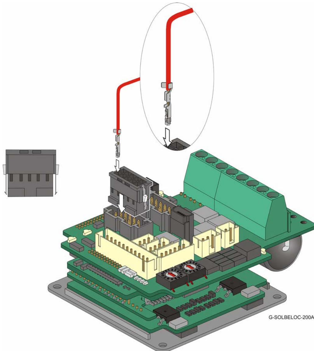
Figure 2: Inserting a wire/pin to the Female Connector
