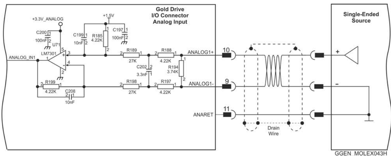
Figure 28: Differential Analog Input
