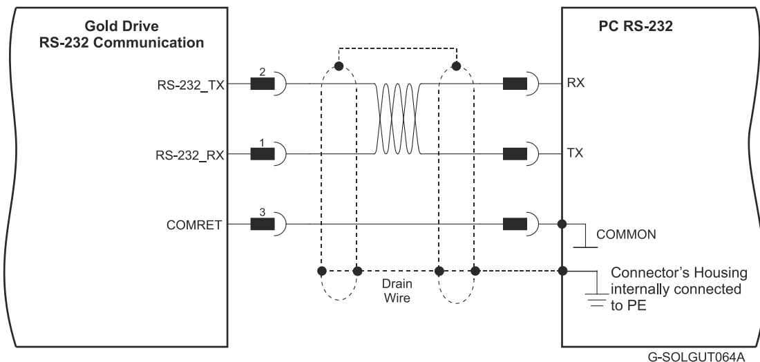
Figure 36: RS-232 Connection Diagram
