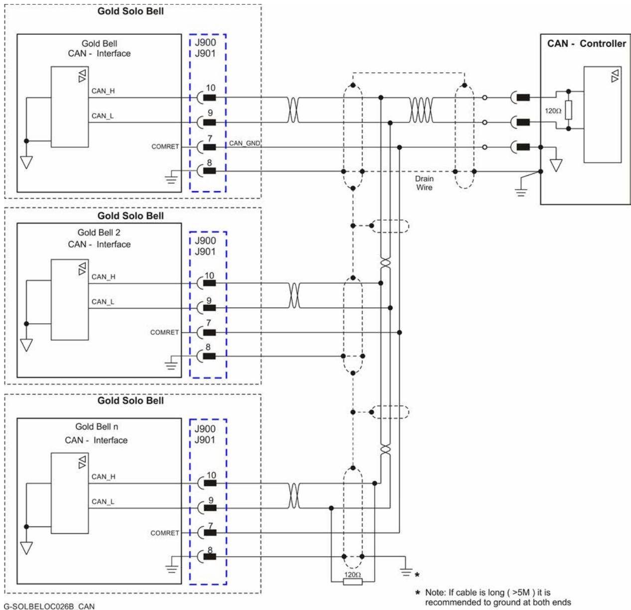
Figure 42: CAN Network Diagram – Drop Off Topology
