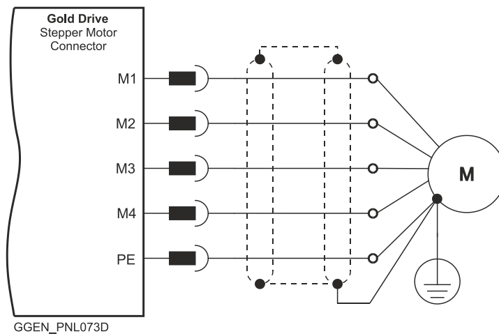
Figure 12: Stepper Motor Power Connection Diagram
