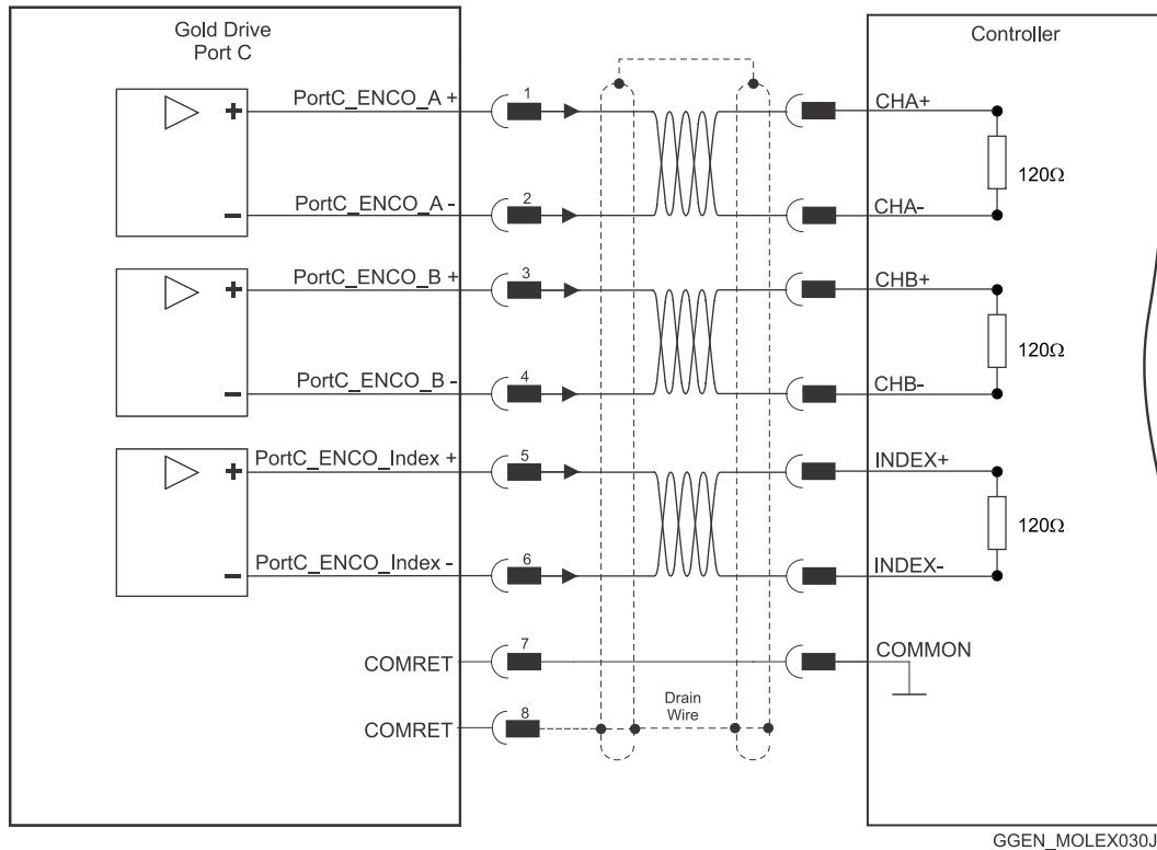
Figure 27: Emulated Encoder Differential Output – Recommended Connection Diagram
