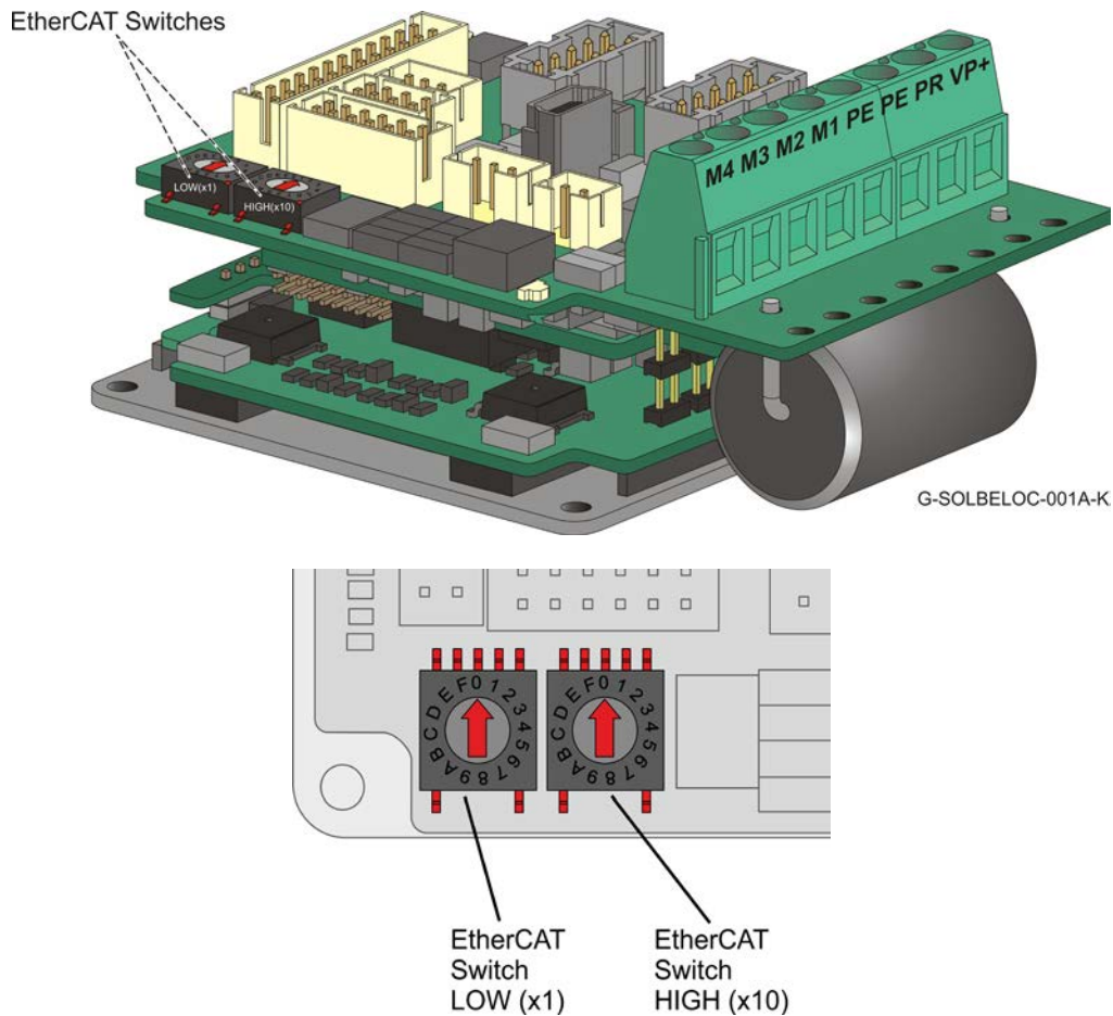
Figure 41: EtherCAT Address Switches
