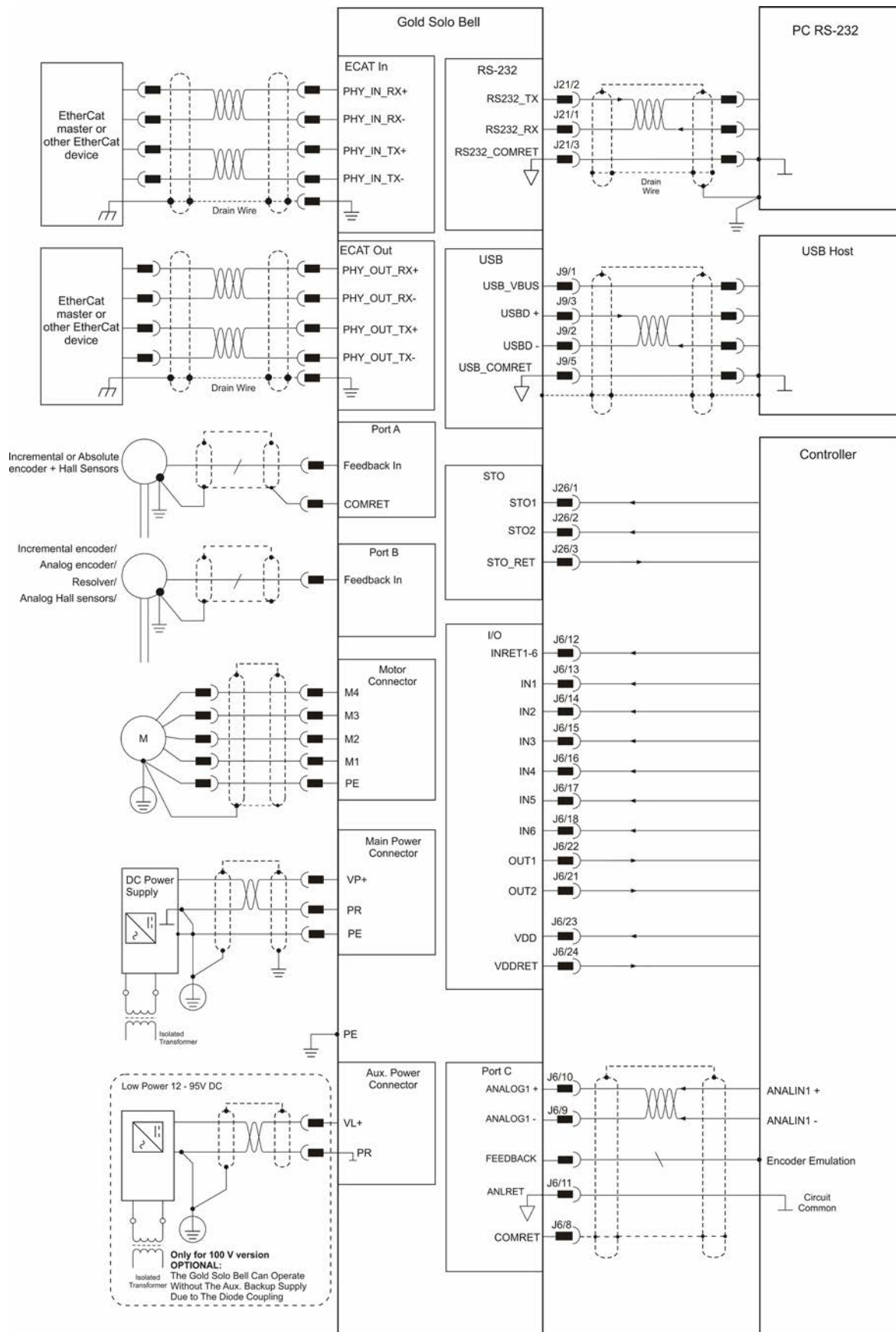
Figure 3: The Gold Solo Bell (2 mm pitch E/C Conn.) Connection Diagram - EtherCAT
