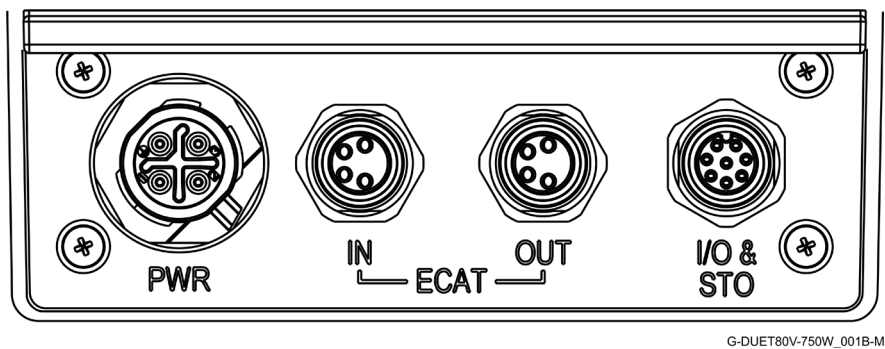
Figure 33: Interface Details
