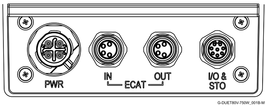
Figure 38: Interface Details
