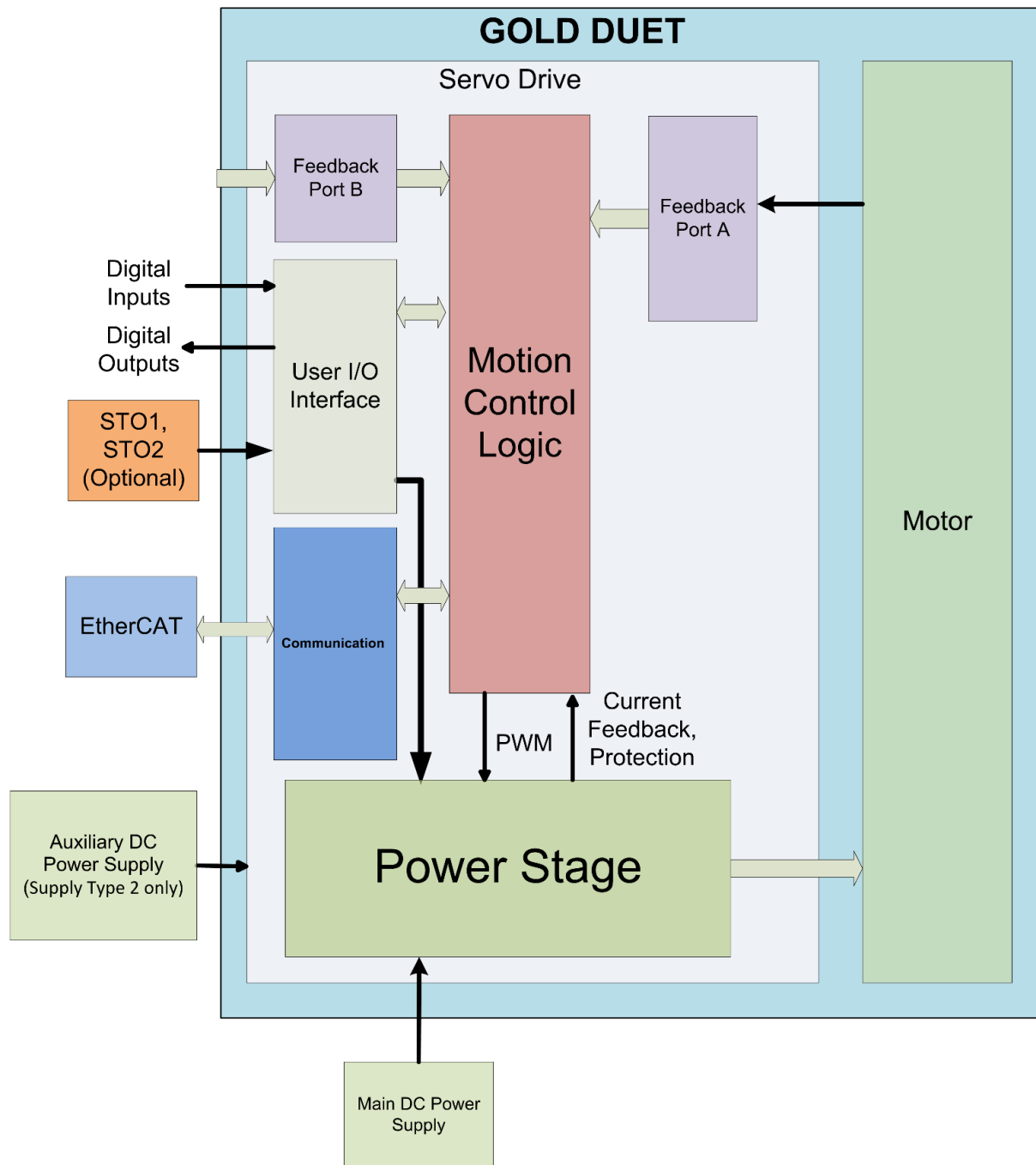
Figure 1: Gold Duet 80 System Block Diagram
