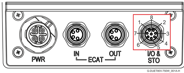
G-DUET-80, 100 Connectors Interface
