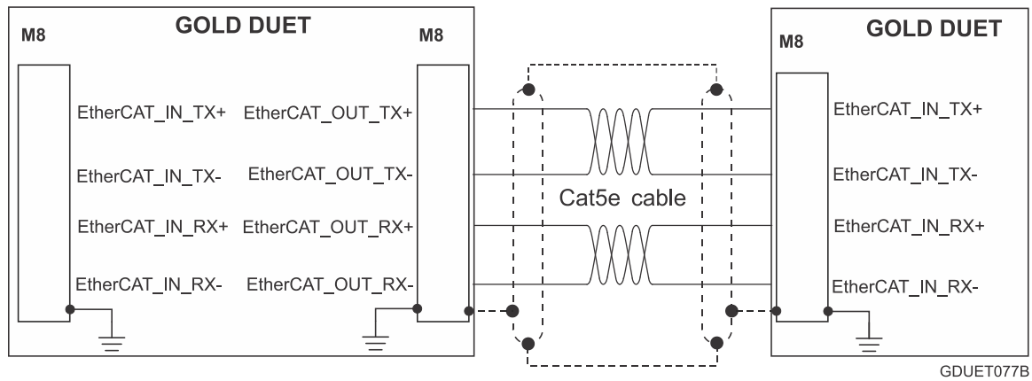
Figure 19: EtherCAT Connections
