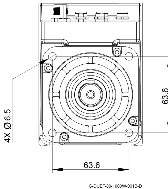
Figure 37: Front View Details and Rotor Shaft/Keyway Details
