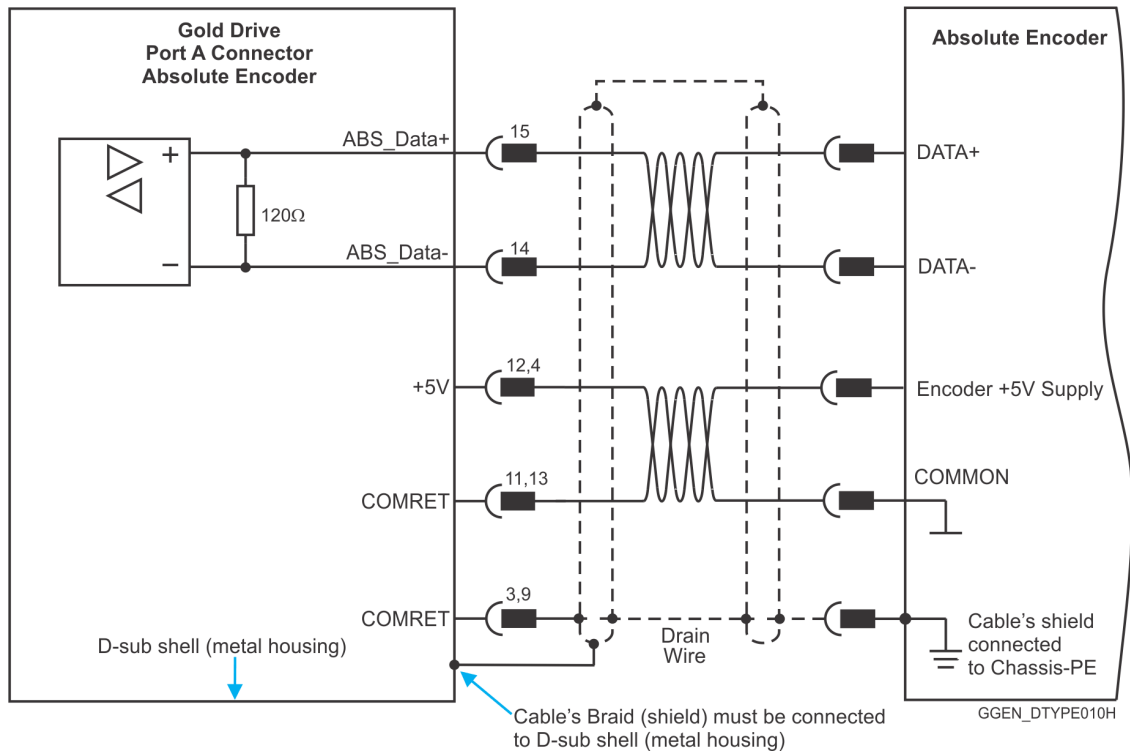
Figure 16: Absolute Serial Encoder – Recommended D-Type Connection Diagram for EnDAT, Biss, and SSI
