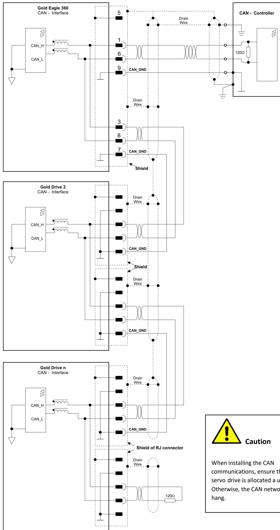
Figure 39: Gold Eagle 360/430 Connection Diagram – CAN
