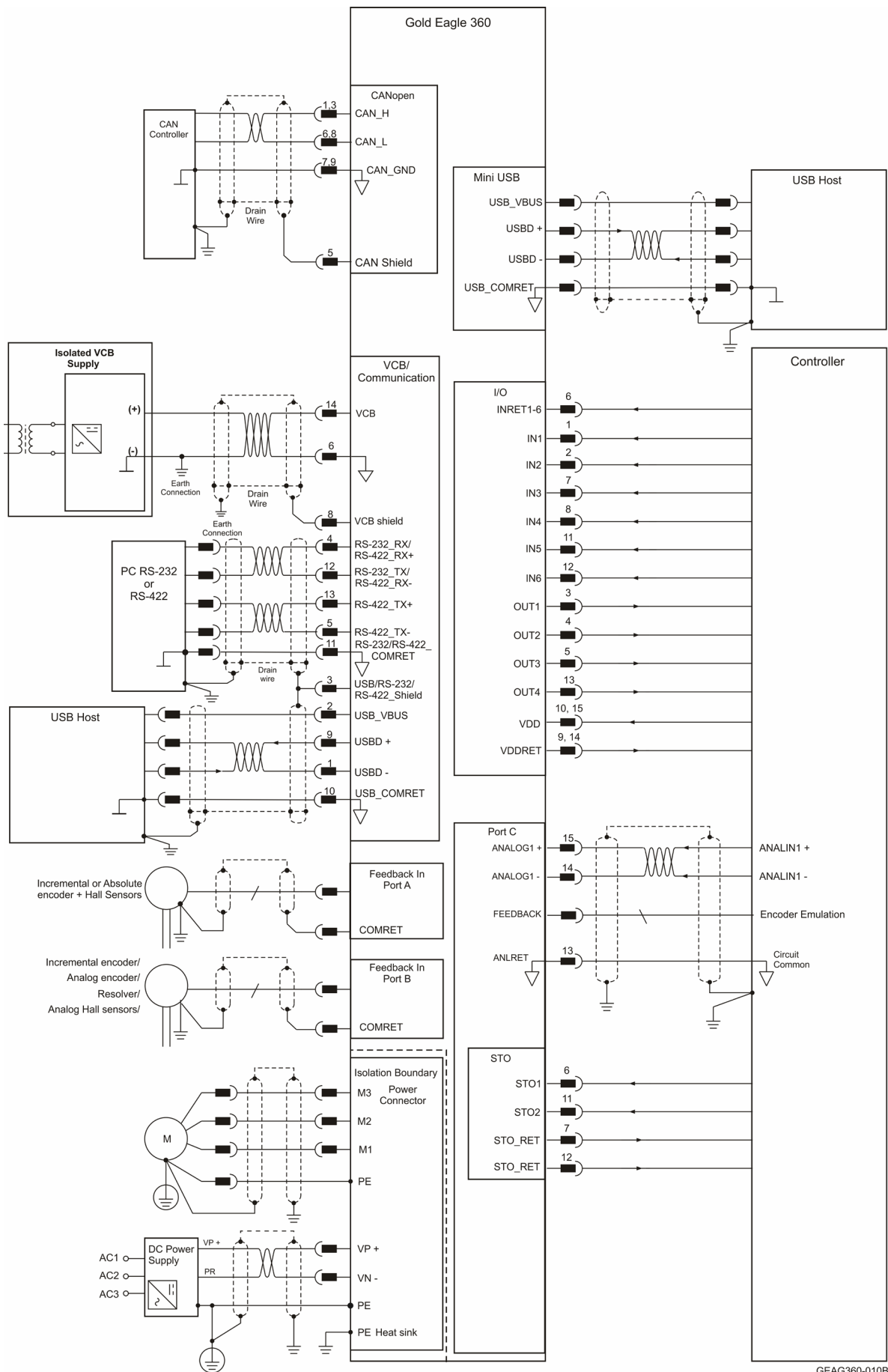
Figure 3: Gold Eagle 360/430 Connection Diagram for CAN
