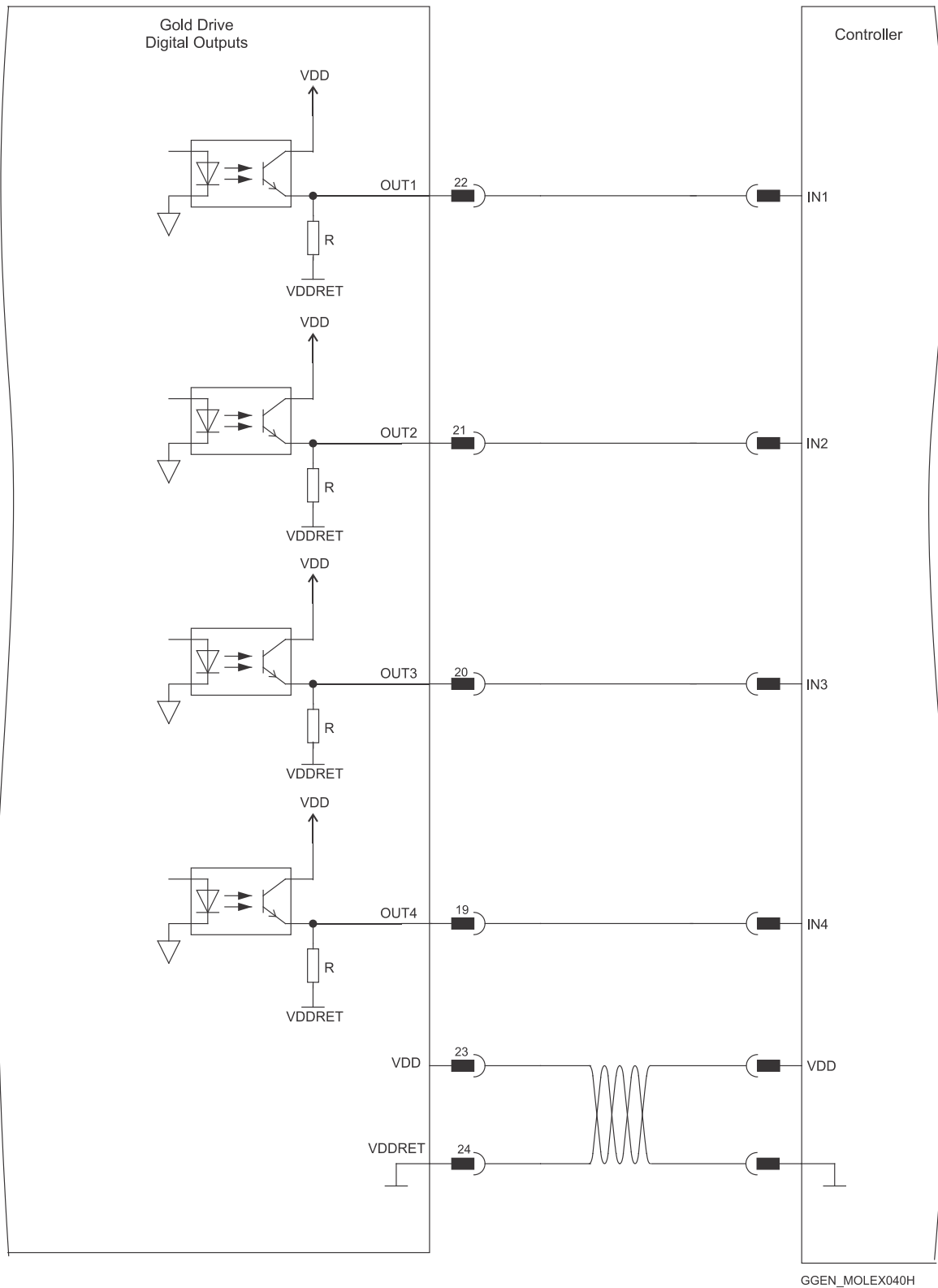
Figure 31: Digital Output Connection Diagram – TTL Option
