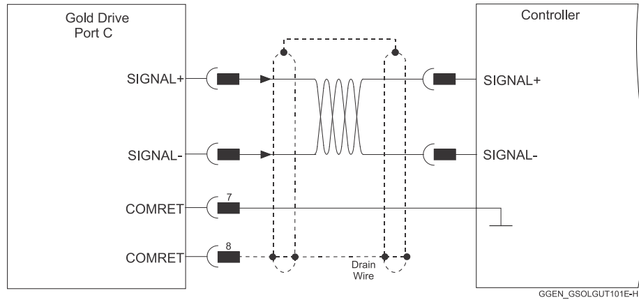
Figure 7: Feedback Port C Cable Assemblies
