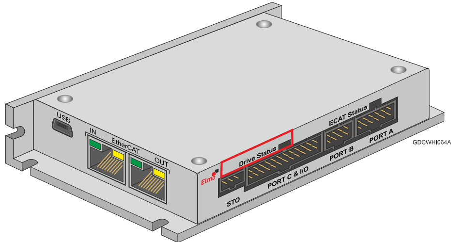
Figure 15: Drive Status Indicator - EtherCAT
