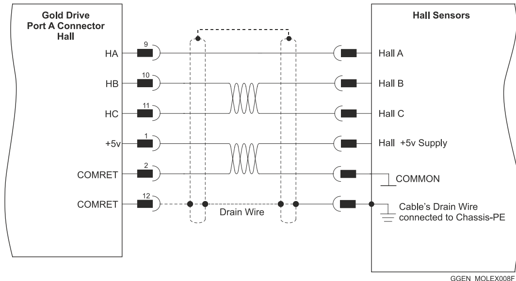
Figure 21: Molex Type Hall Sensors Connection Diagram
