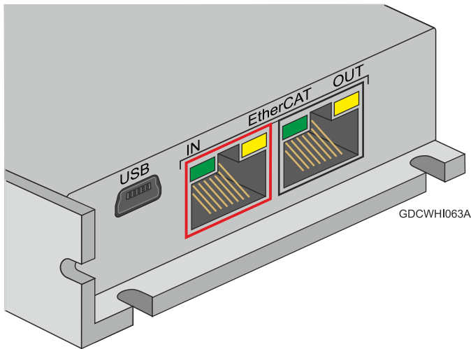
8-Pin RJ-45
