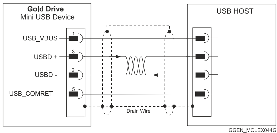
Figure 36: USB Network Diagram
