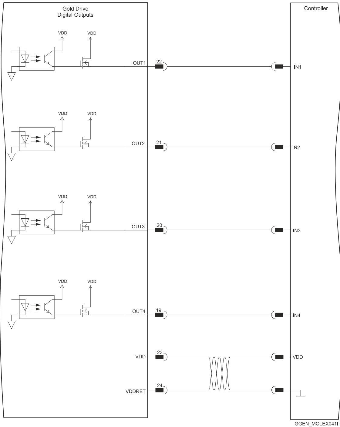
Figure 33: Digital Output Connection Diagram – Source PLC Option
