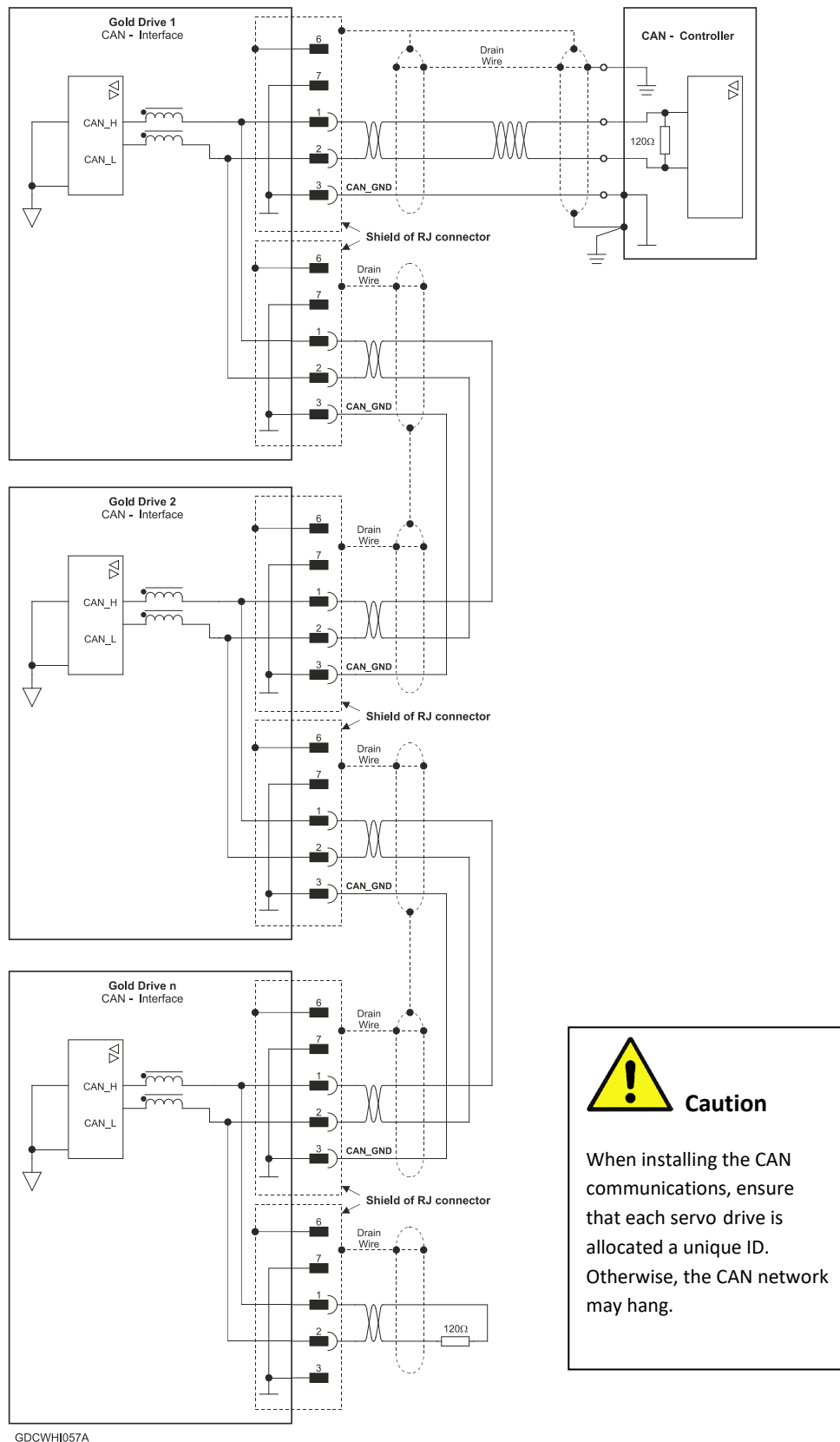
Figure 40: Gold DC Whistle Connection Diagram – CAN
