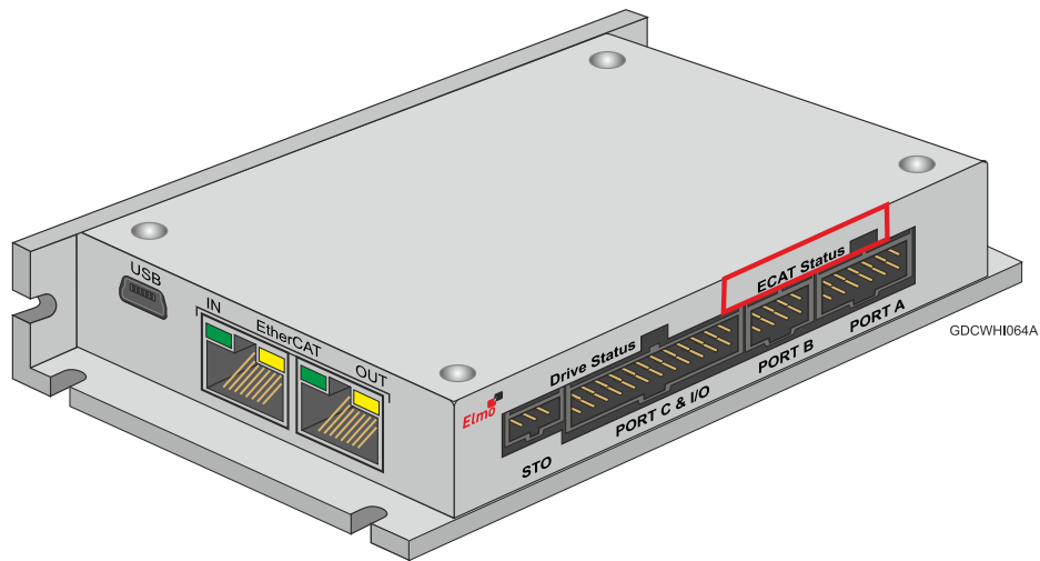
Figure 38: EtherCAT Status LED
