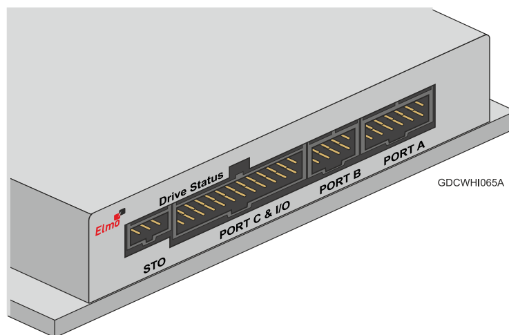
Figure 39: Gold DC Whistle Status Indicator - CAN
