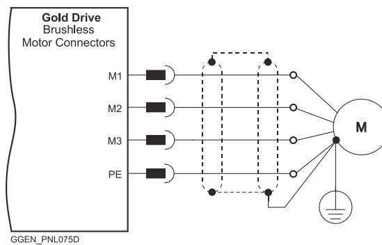
Figure 10: Brushless Motor Power Connection Diagram
