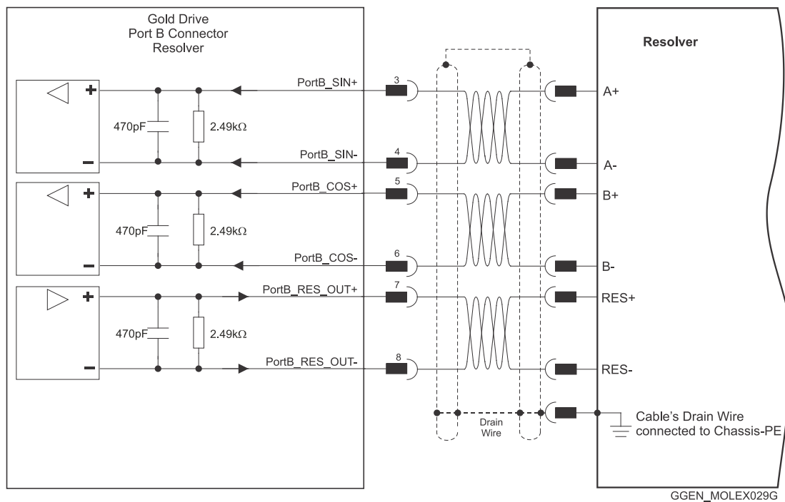
Figure 27: Port B – Resolver Molex Type Connection Diagram
