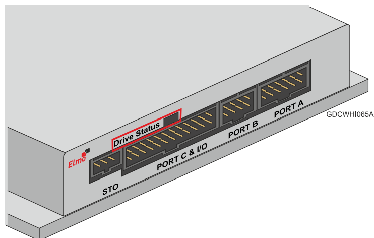
Figure 16: Drive Status Indicator - CAN
