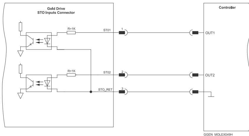
Figure 18: STO Input Connection – TTL Option
