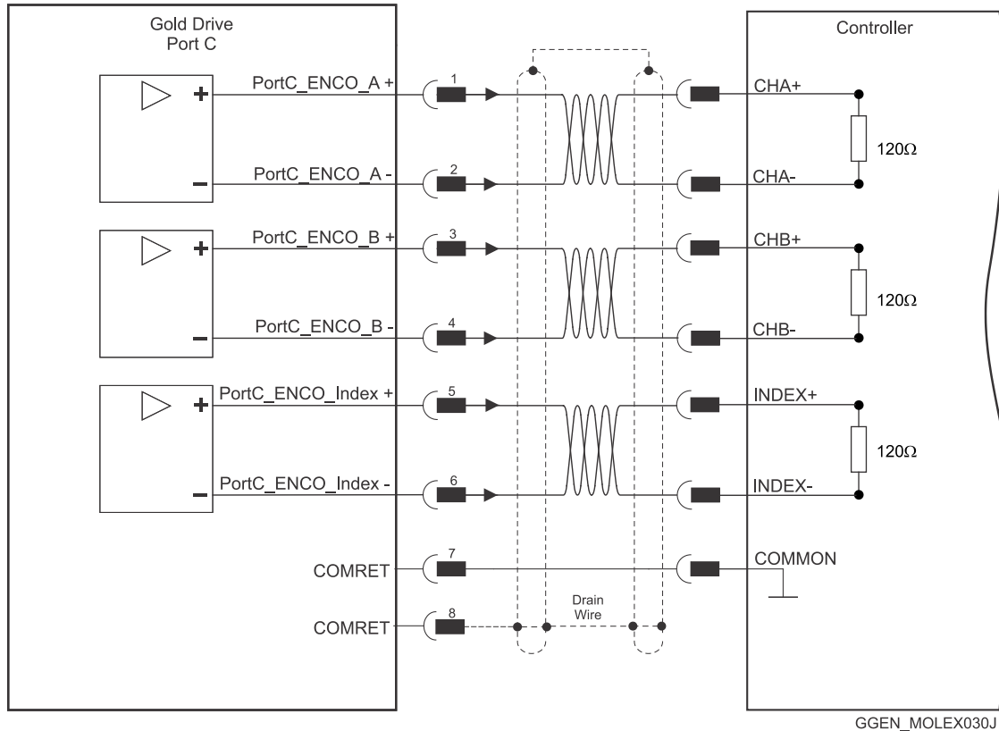
Figure 28: Emulated Encoder Differential Output – Recommended Connection Diagram
