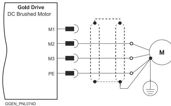
Figure 11: Brushed Motor Power Connection Diagram
