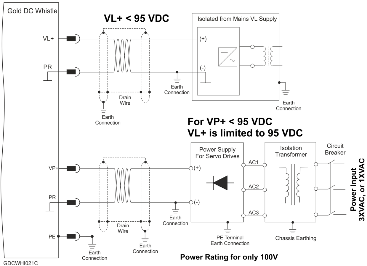
Figure 14: Control Power Supply Connections Diagram
