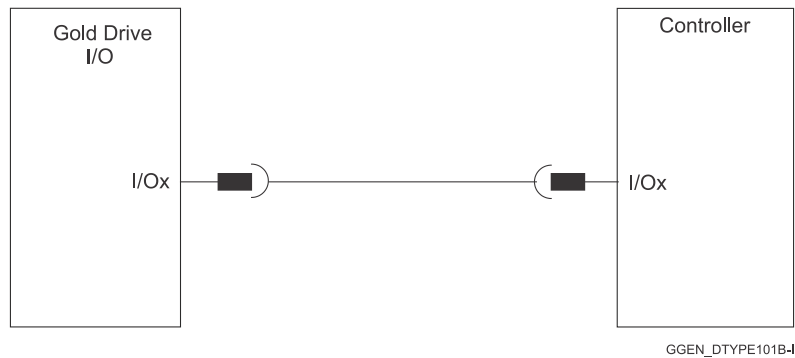
Figure 8: Feedback IO Cable Assemblies
