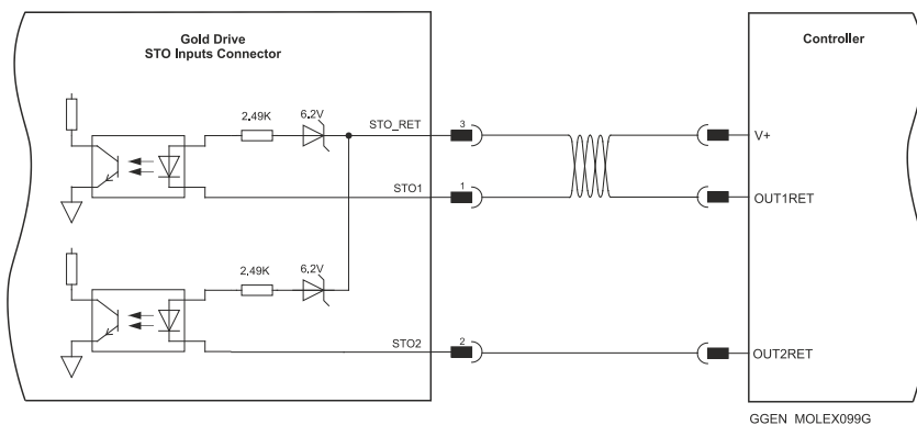
Figure 19: STO Input Connection – Sink Option
