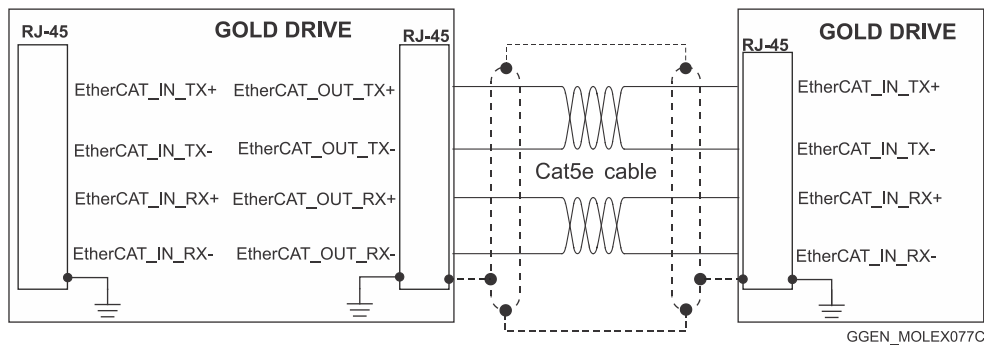
Figure 37: EtherCAT RJ-45 Connections
