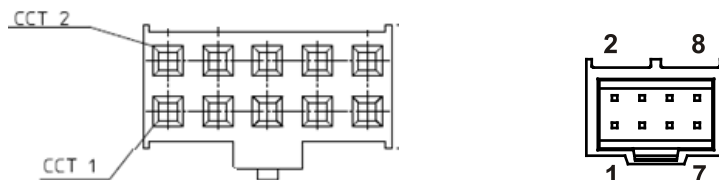
Figure 4: Molex vs Elmo Technical Diagram Examples Showing Pinout Numbers
