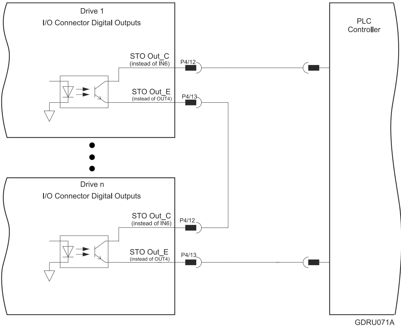
Figure 29: STO Output
