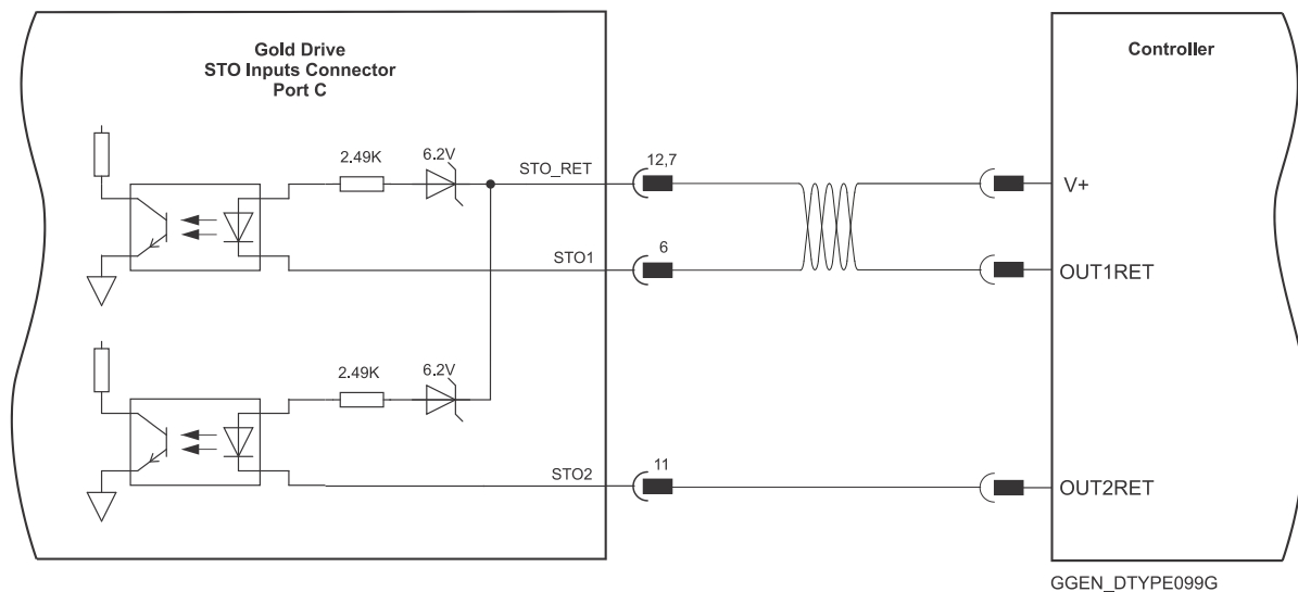
Figure 28: STO D-Type Input Connection – Sink Option
