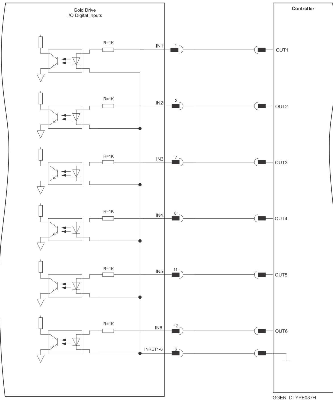
Figure 30: Digital Input TTL Mode D-Type Connection Diagram
