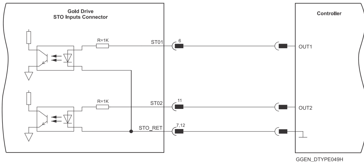
Figure 27: STO Input Connection – TTL Option
