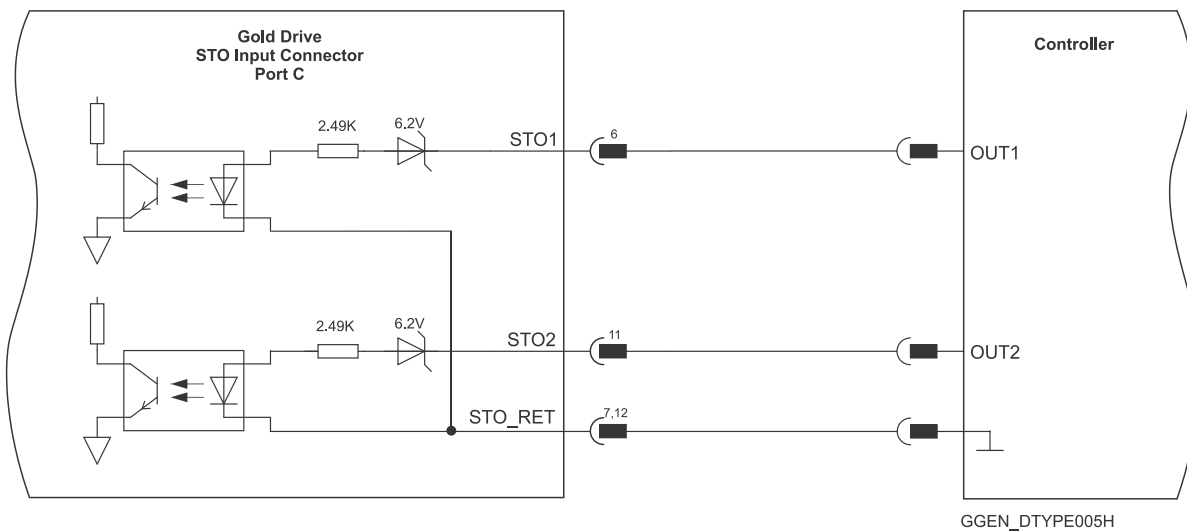
Figure 26: STO Input Connection – PLC Source Option
