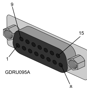
15-Pin D-Type Female Connector
