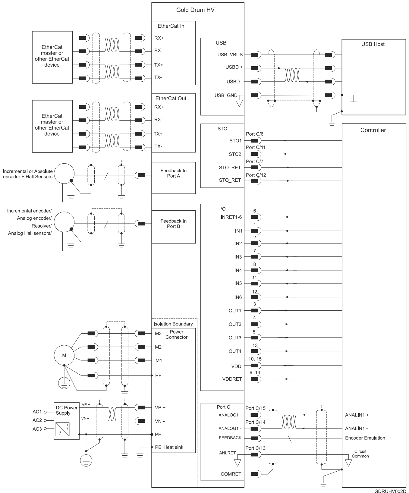
Figure 3: Gold Drum HV (High Voltage) Connection Diagram for EtherCAT – 400 V without Power Supply Backup Functionality for 0 or 1 Options
