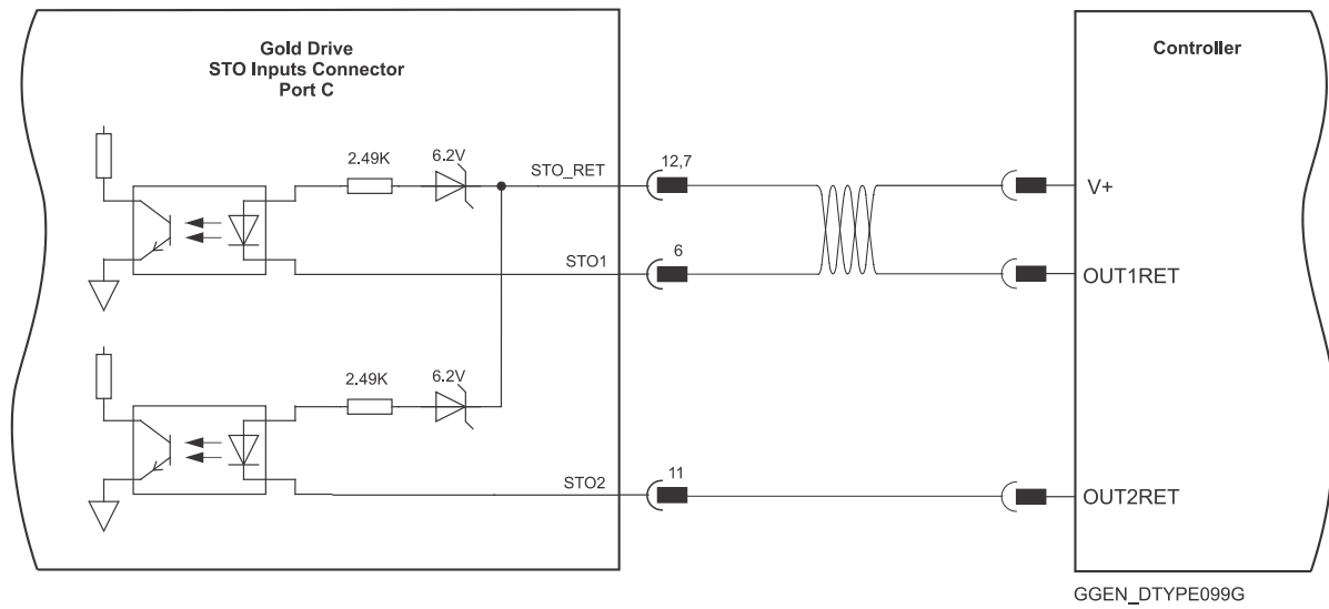
Figure 29: STO D-Type Input Connection – Sink Option
