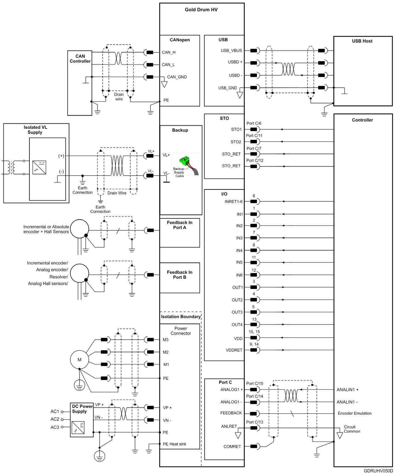
Figure 4: Gold Drum HV (High Voltage) Connection Diagram for CAN – with Power Supply Backup Functionality (H, S, T, or A Option)
