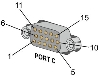
15-Socket High Density D-Type Connector
