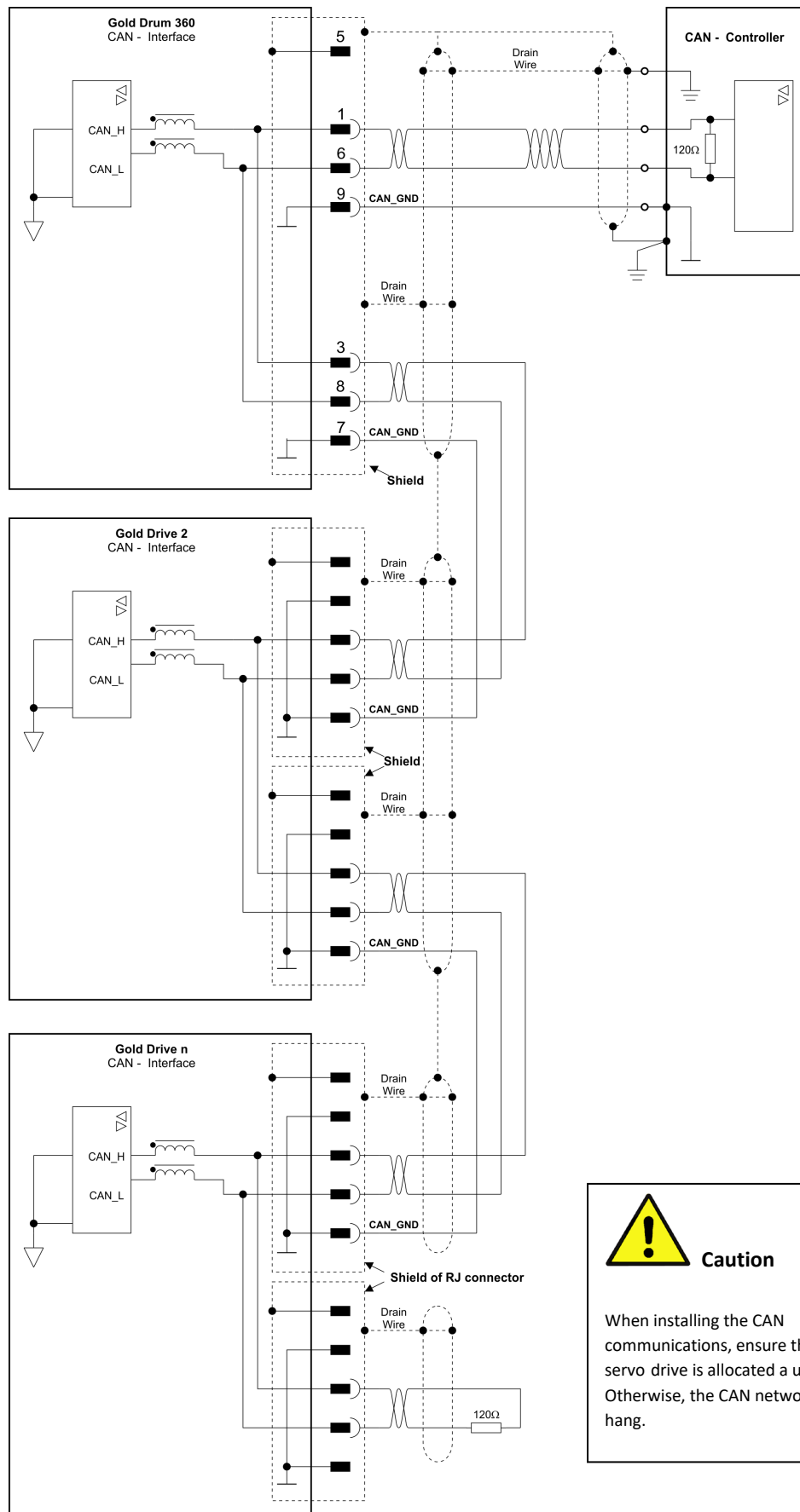
Figure 39: Gold Drum 360/430 Connection Diagram – CAN
