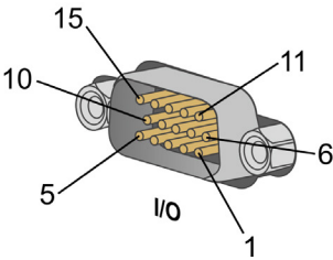
15-Pin High Density D-Type Male Connector
