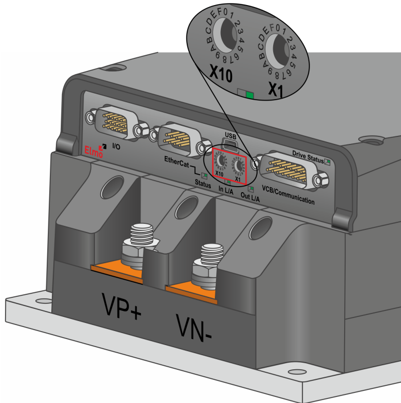
Figure 38: Position of EtherCAT Address Switches on Gold Drum 360/430
