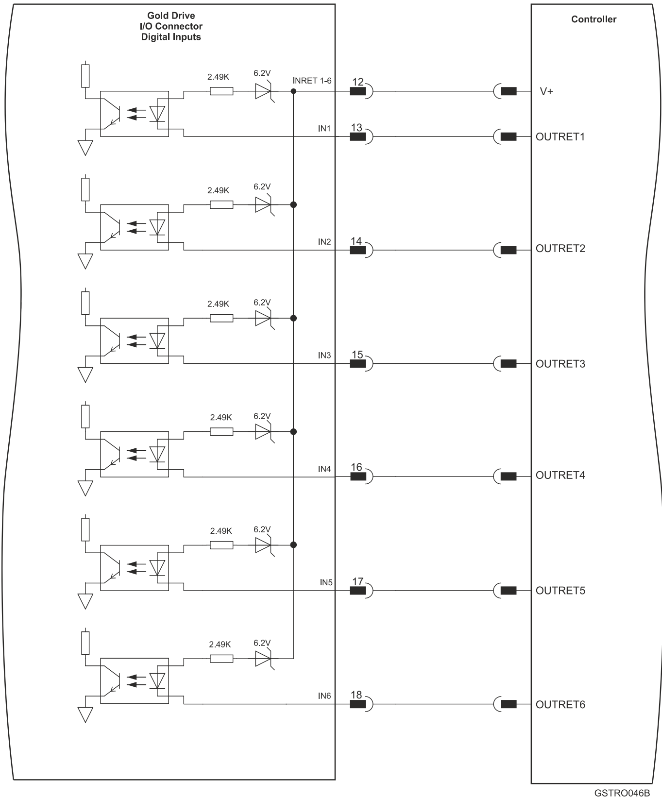
Figure 33: Digital Input Sink Mode – PLC voltage level Shrouded Type Connection Diagram
