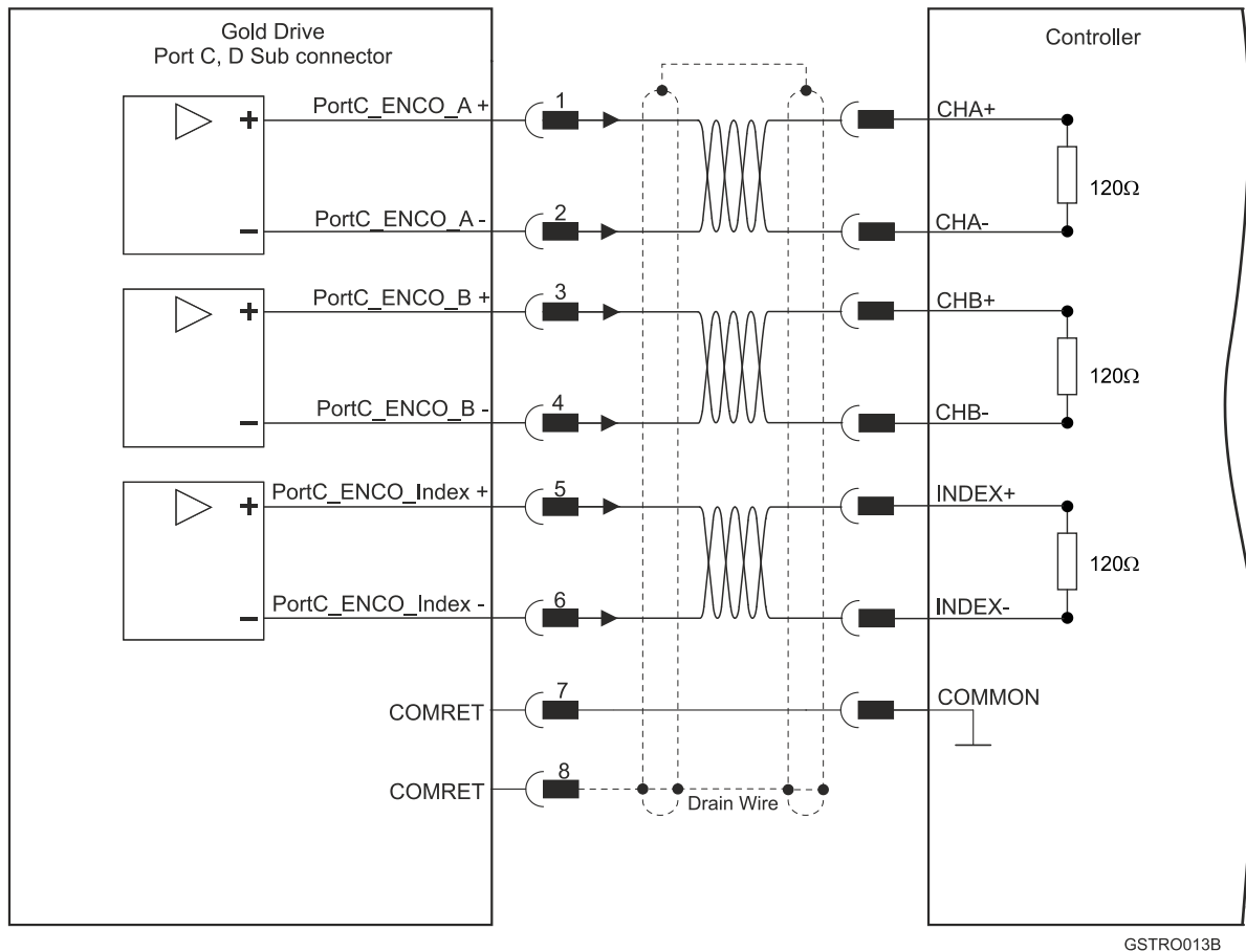
Figure 27: Emulated Encoder Differential Output – Recommended Shrouded Type Connection Diagram
