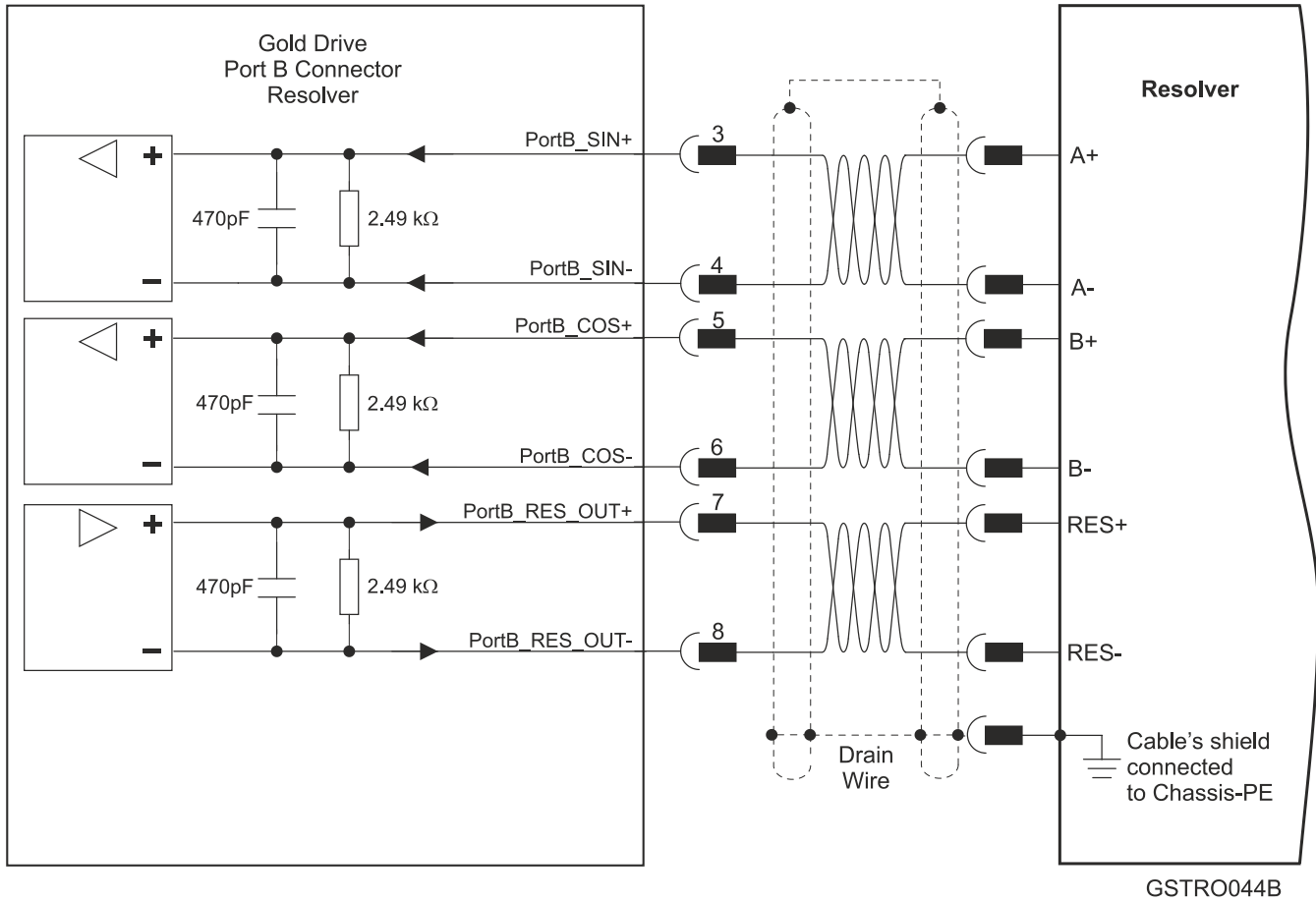
Figure 26: Port B – Resolver Shrouded Type Connection Diagram
