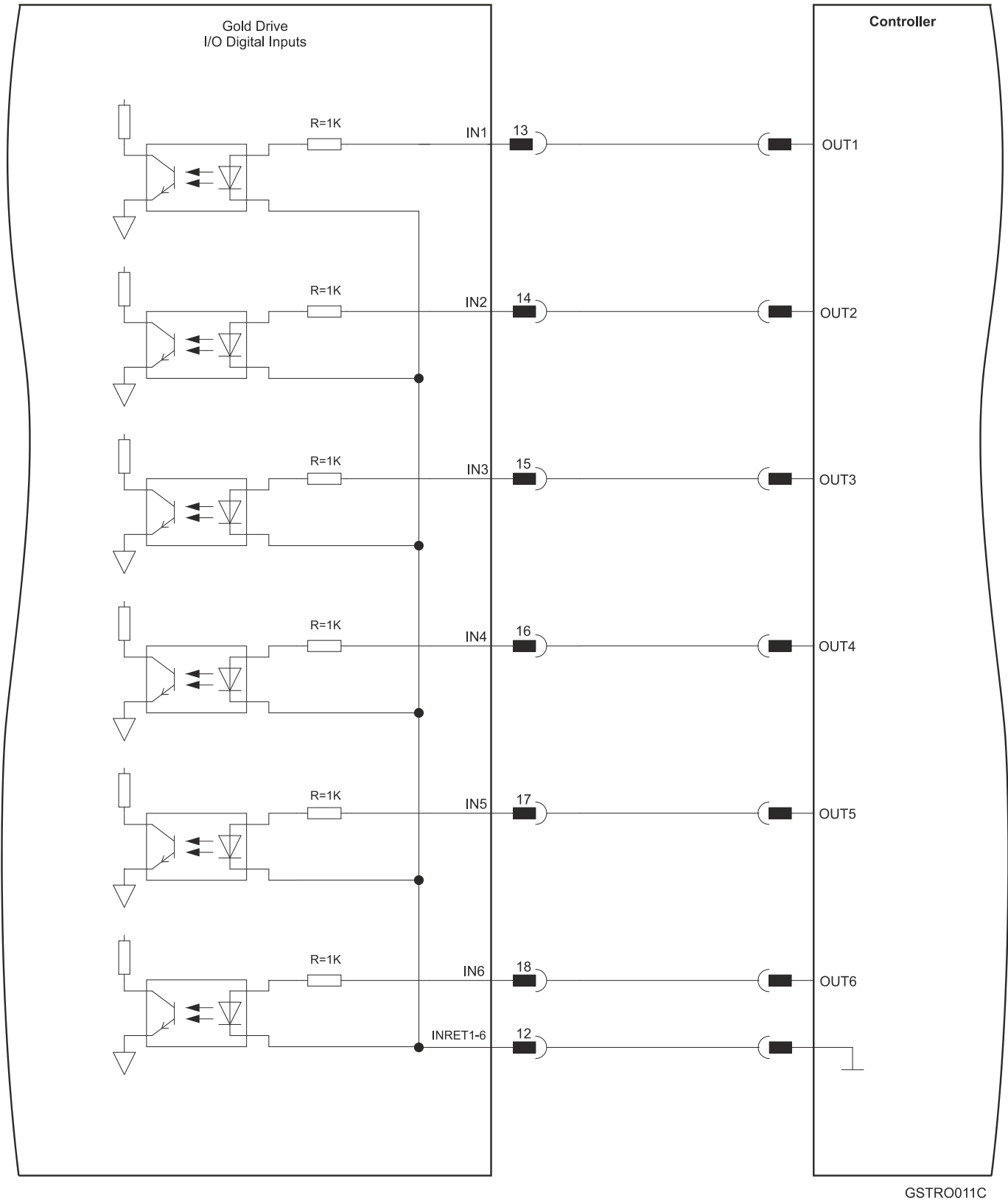
Figure 29: Digital Input TTL Mode Shrouded Type Connection Diagram
