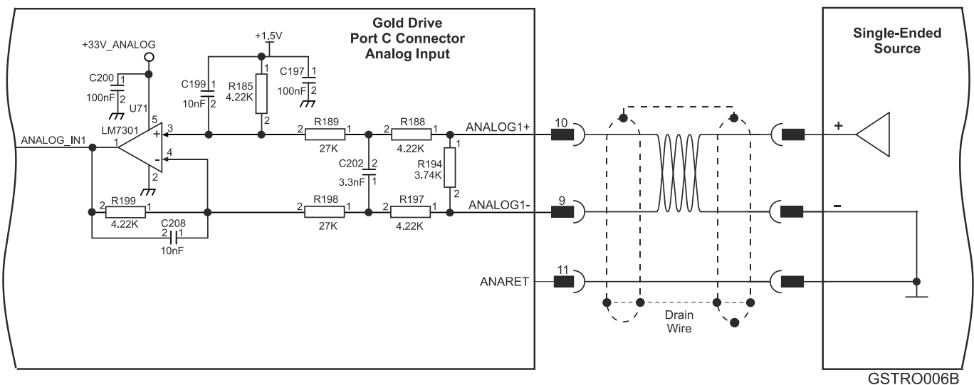
Figure 28: Differential Analog Shrouded Type Input
