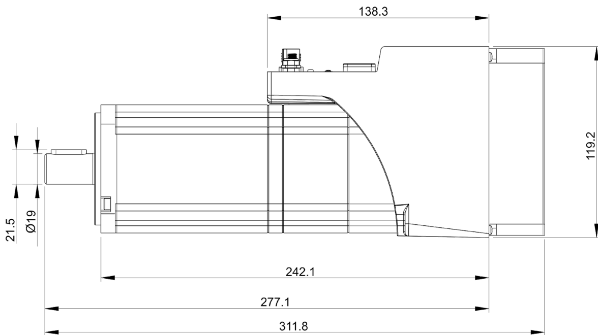
Figure 30: Side View Details
