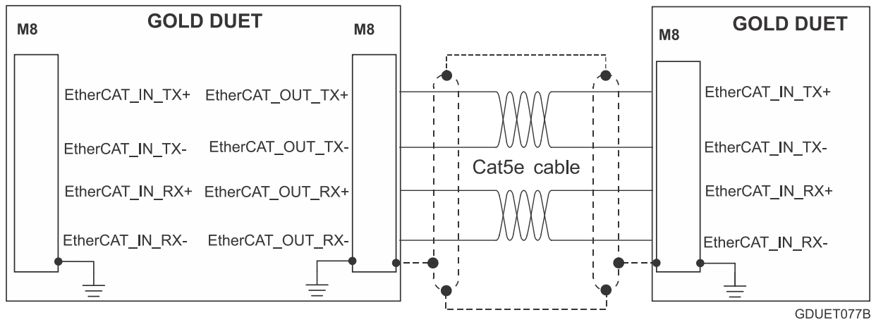
Figure 19: EtherCAT Connections
