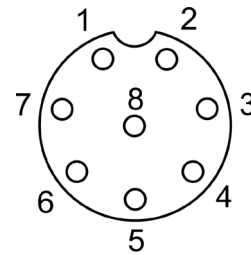
G-DUET-80, 100 Connectors Interface
