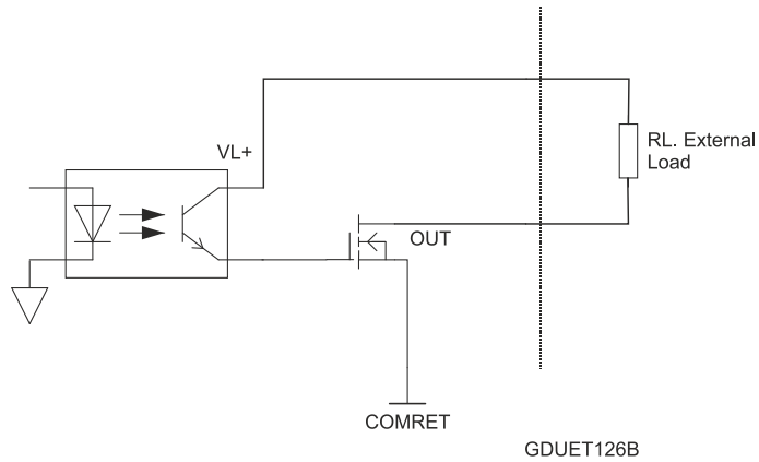
Figure 17: Digital Output PLC Sink Schematic
