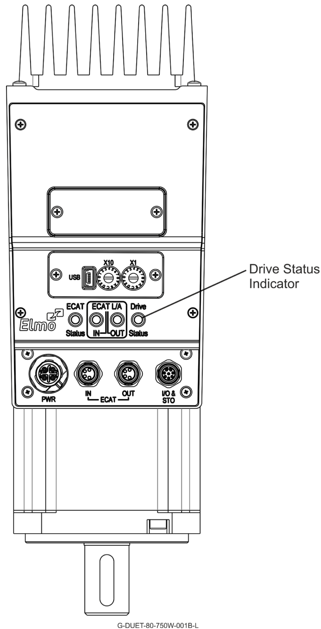
Figure 4: LED Indicators
