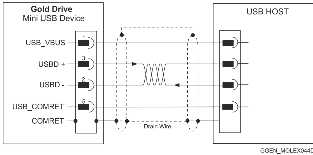
Figure 23: USB Network Diagram
