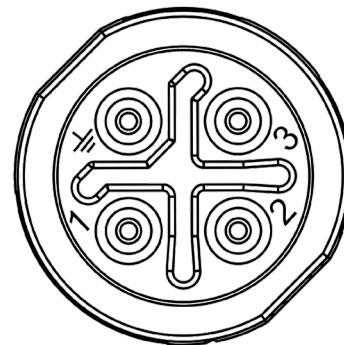
Figure 5: M12 socket 4-pos S-encoded Power Male Connector and interface
