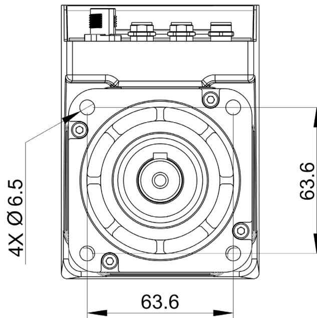
Figure 26: Top View Details
