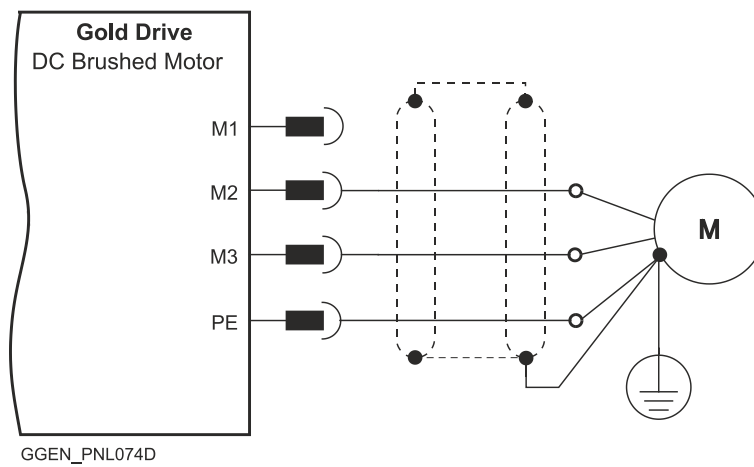
Figure 10: DC Brushed Motor Power Connection Diagram
