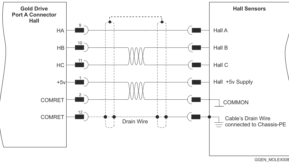
Figure 19: Shrouded Type Hall Sensors Connection Diagram
