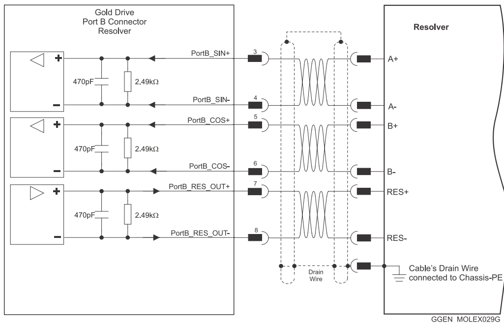
Figure 25: Port B – Resolver Shrouded Type Connection Diagram
