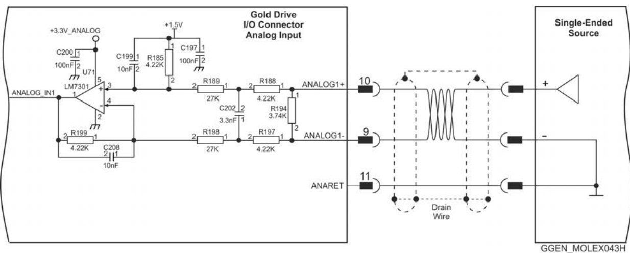
Figure 27: Differential Analog Input
