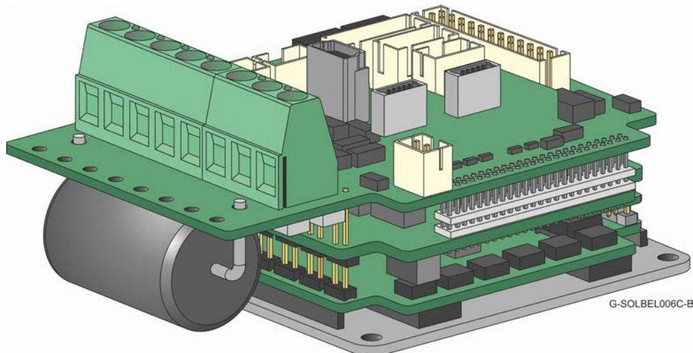
Figure 38: Gold Solo Bell (1 mm pitch E/C Conn.) - CAN
