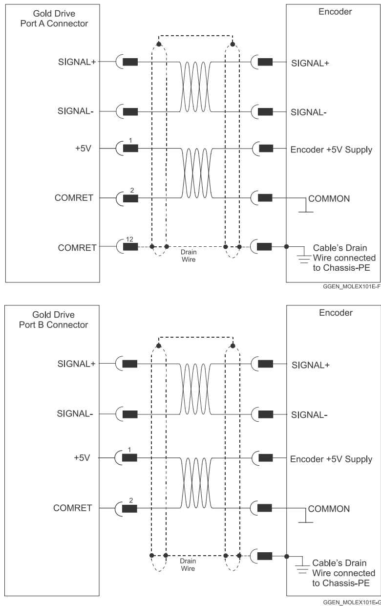
Figure 5: Feedback Port A and B Cable Assemblies
