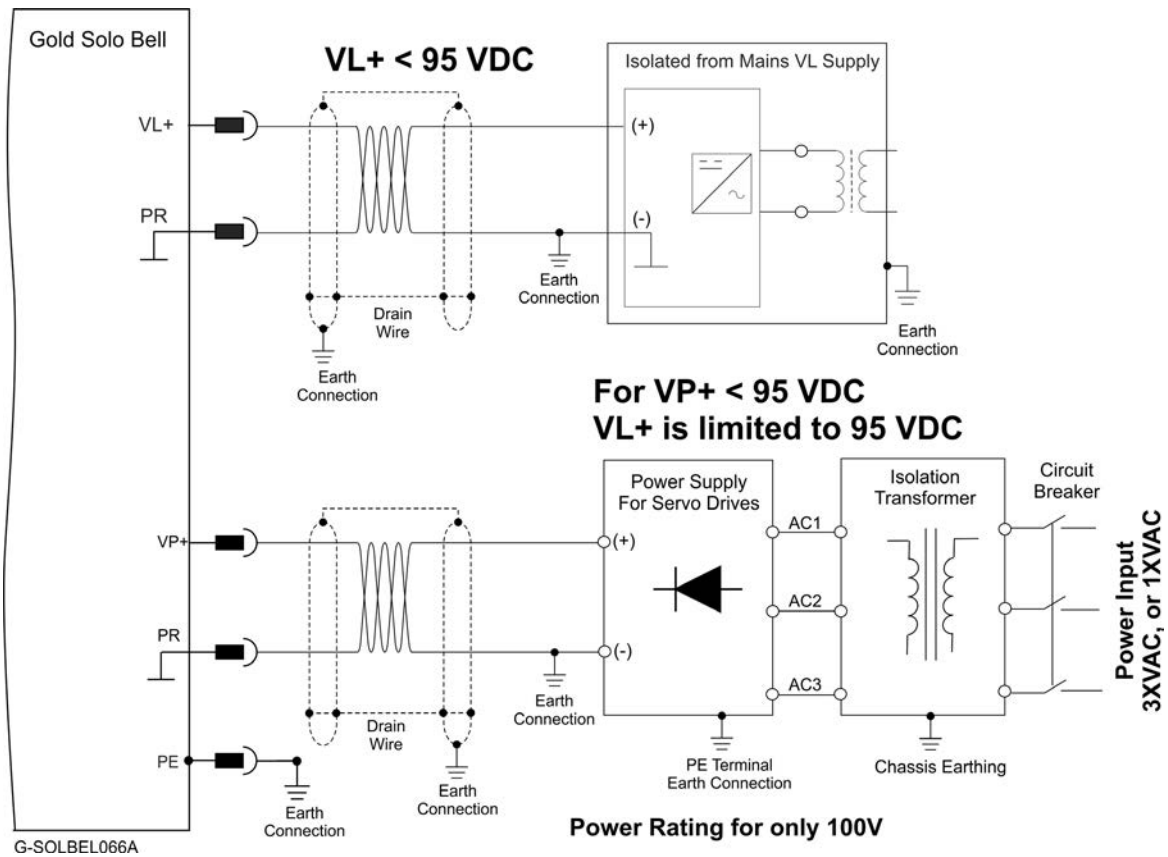
Figure 14: Control Supply Connection Diagram
