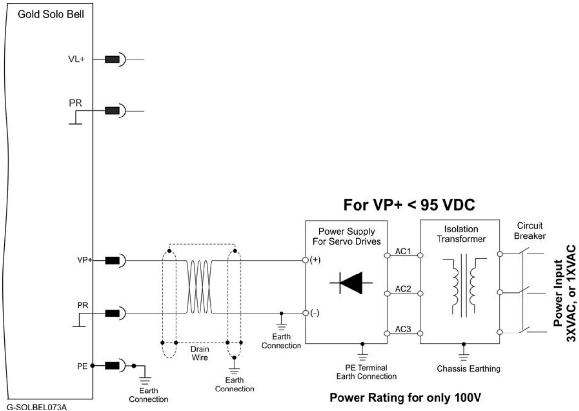
Figure 13: Main Power Supply Connection Diagram (No Control Supply)
