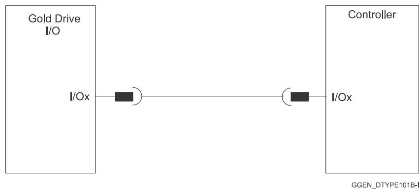
Figure 7: Feedback IO Cable Assemblies
