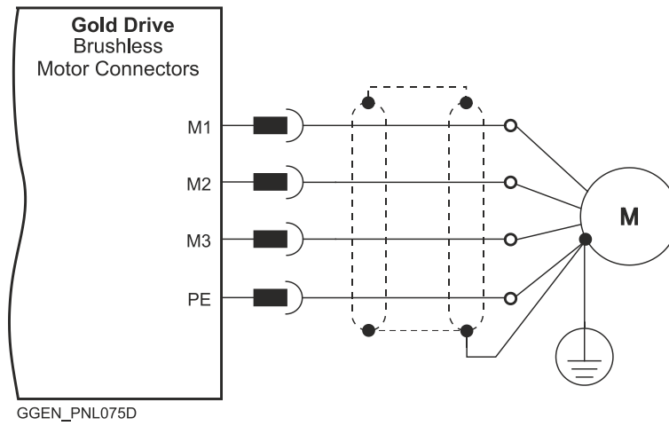
Figure 9: Brushless Motor Power Connection Diagram
