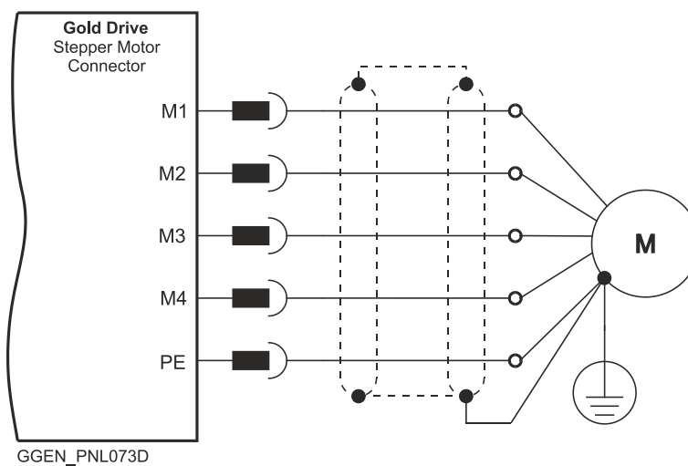
Figure 11: Stepper Motor Power Connection Diagram
