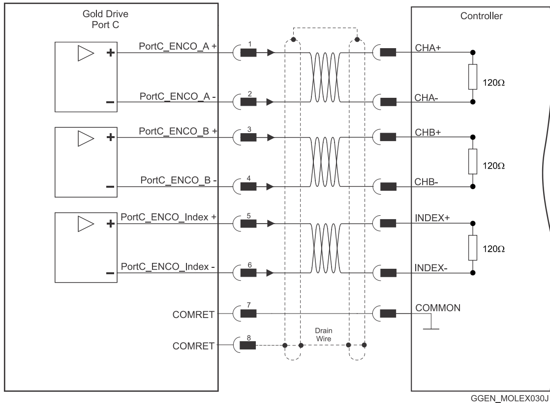
Figure 26: Emulated Encoder Differential Output – Recommended Connection Diagram
