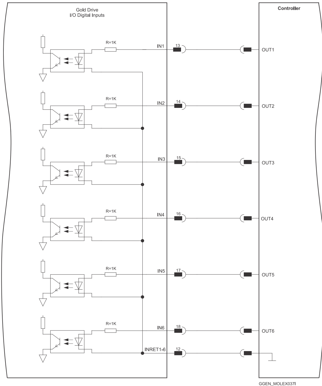
Figure 28: Digital Input TTL Mode Connection Diagram
