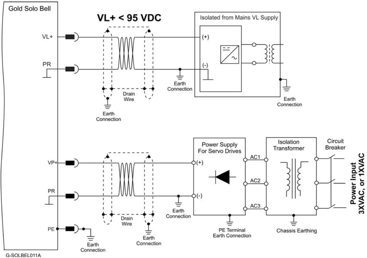
Figure 12: 200 VDC Power Source Connection Diagram
