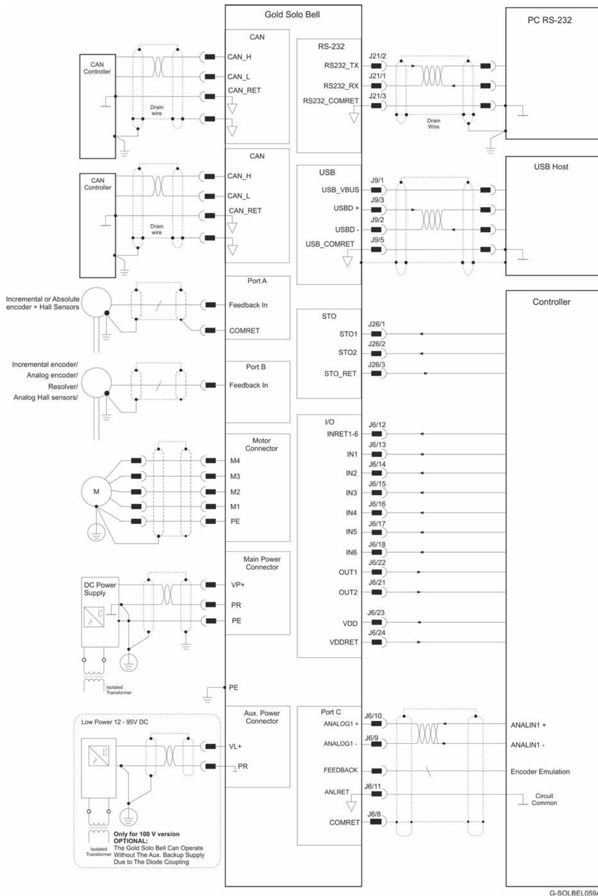
Figure 3: The Gold Solo Bell (1 mm pitch E/C Conn.) Connection Diagram – CAN
