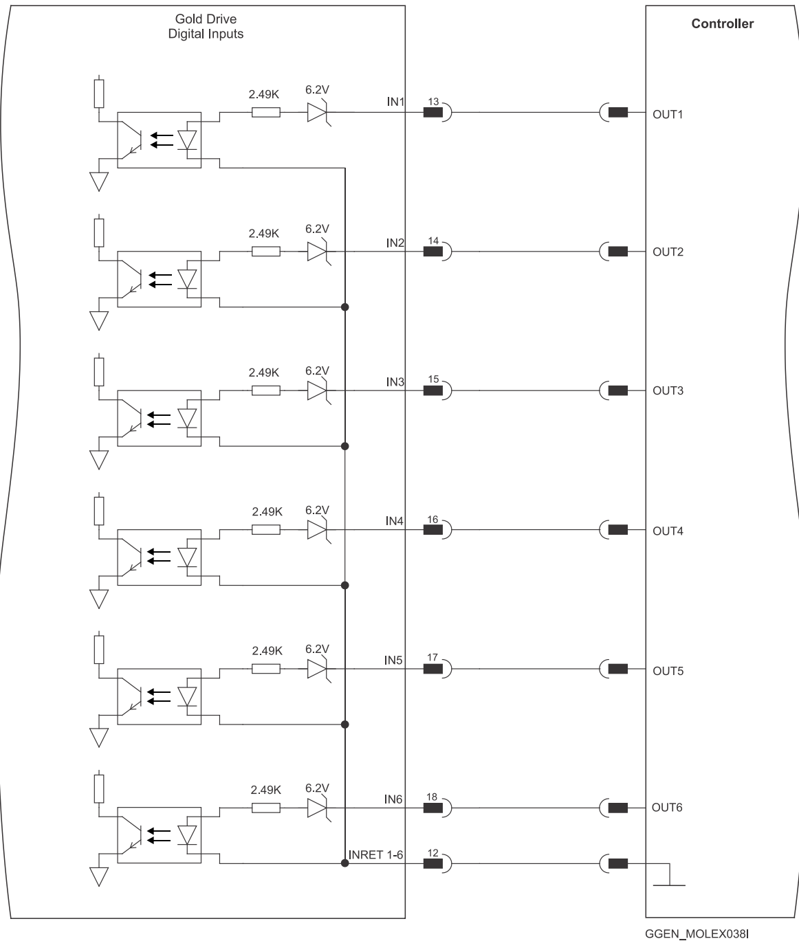
Figure 30: Digital Input Connection Diagram – Source PLC Option
