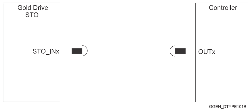
Figure 8: STO Cable Assemblies
