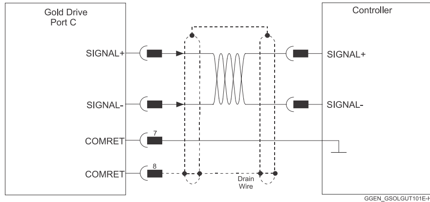
Figure 6: Feedback Port C Cable Assemblies
