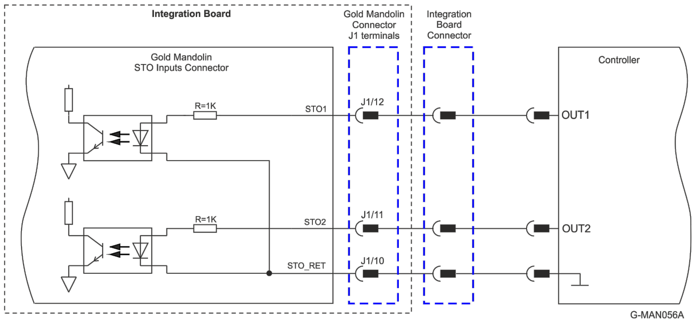
Figure 32: STO Input Connection – TTL Option
