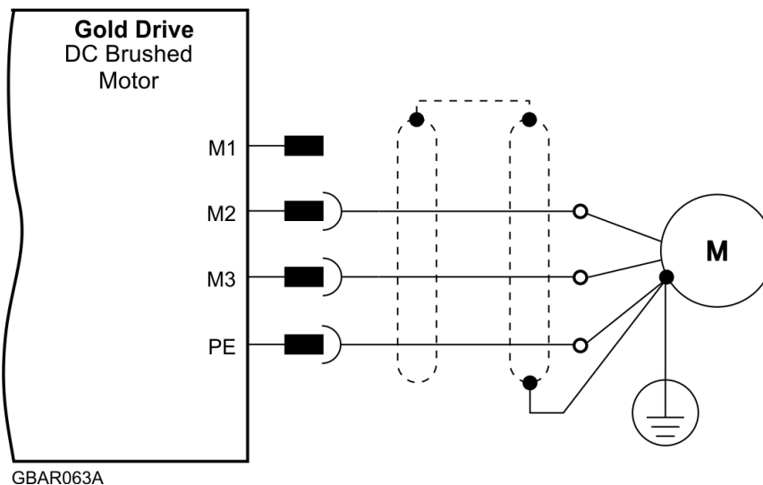
Figure 7: Brushed Motor Power Connection Diagram
