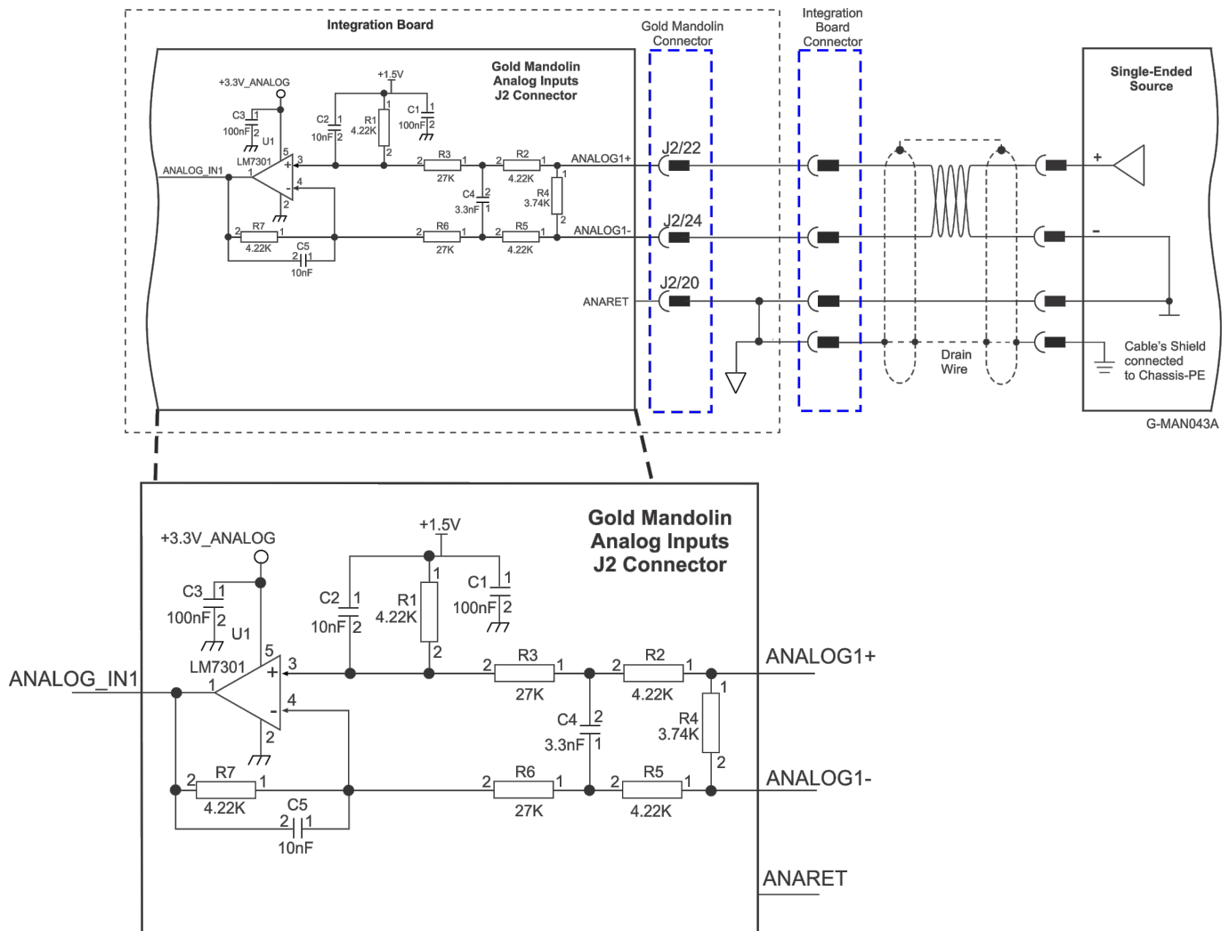
Figure 24: Analog Input with Differential \pm 10 V
