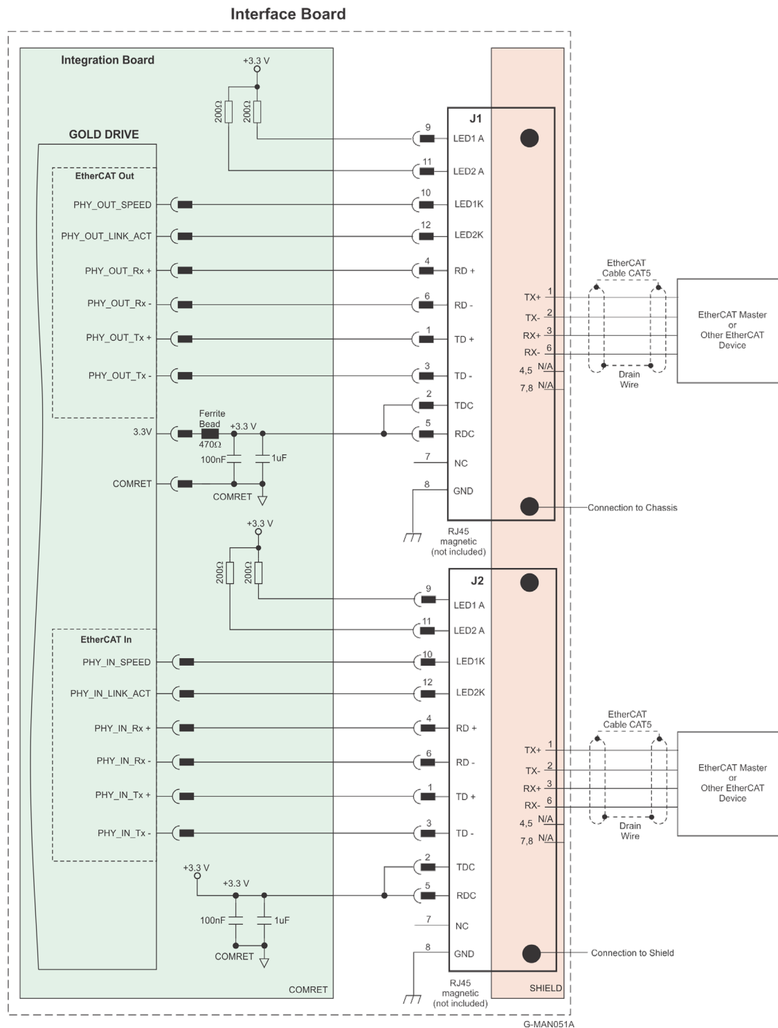
Figure 28: EtherCAT Connection Schematic with Diagram Sign of 3.3V
