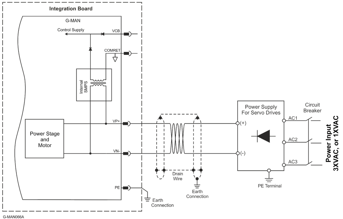
Figure 13: Gold Mandolin Single supply Topology
