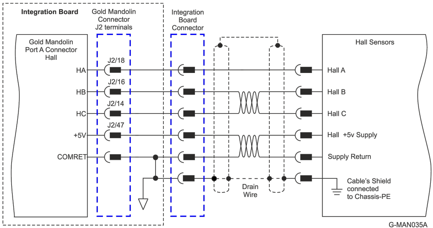
Figure 16: Hall Sensors Connection Diagram
