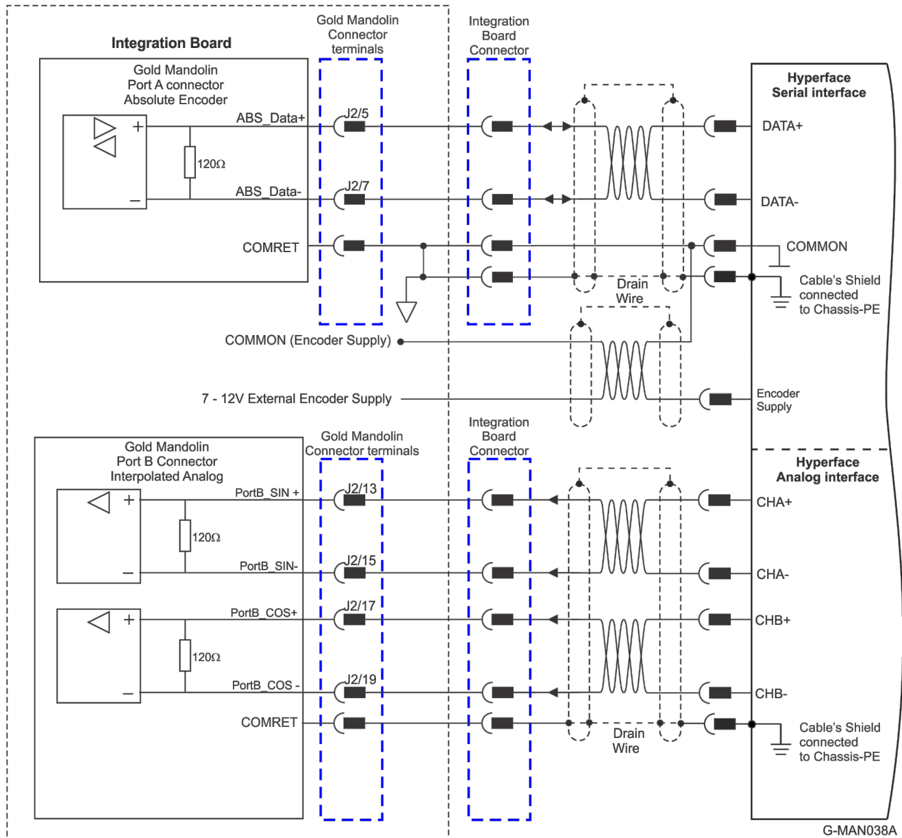
Figure 19: Absolute Serial Encoder – Recommended Connection Diagram for Stegmann Hiperface
