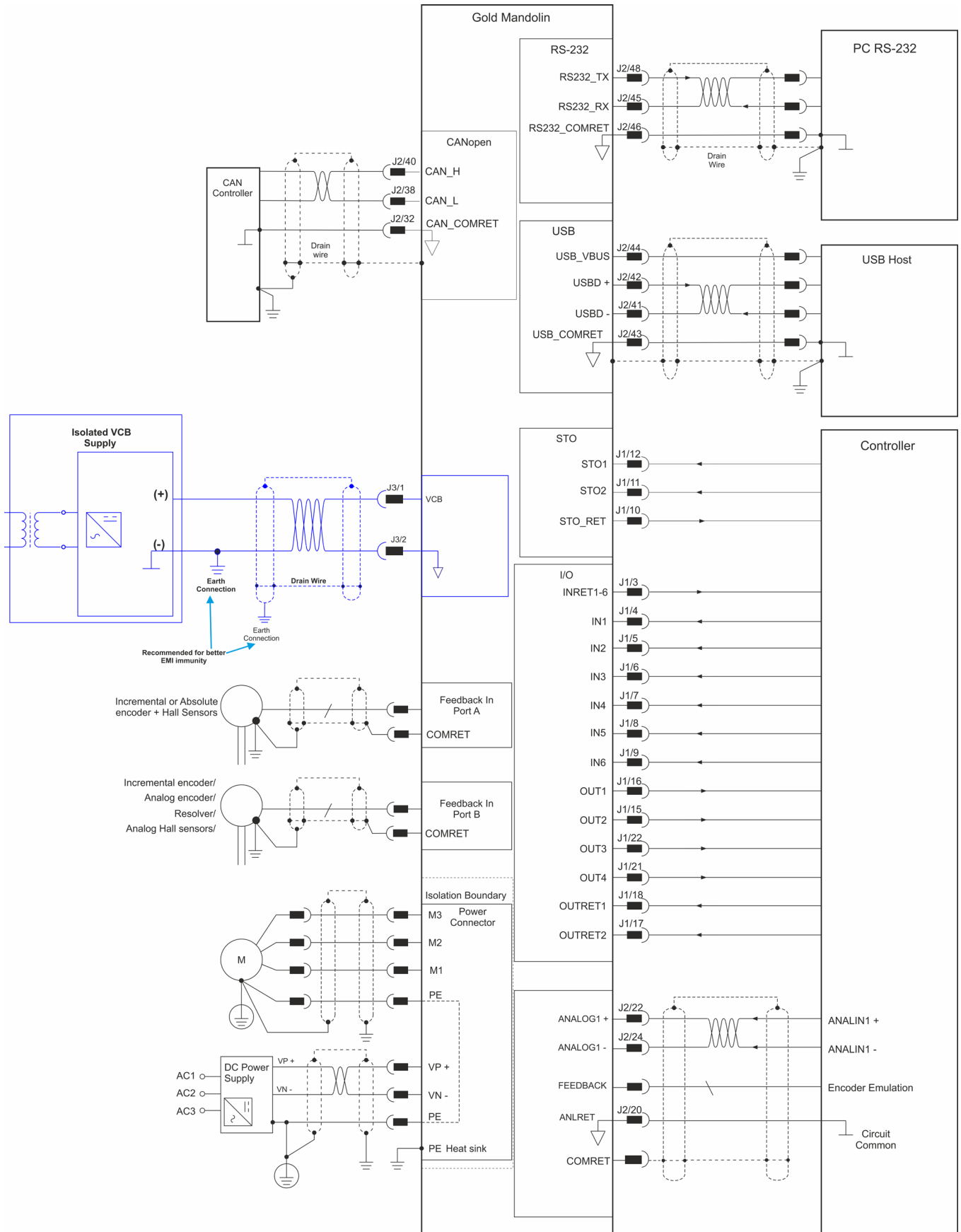
Figure 5: Gold Mandolin Connection Diagram for CAN
