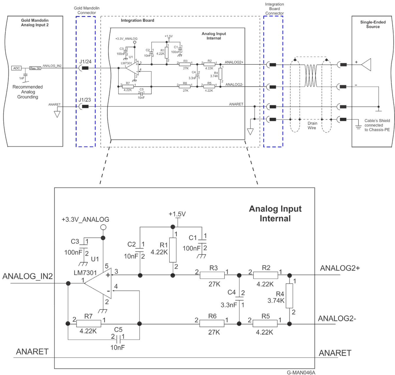
Figure 25: Analog Input 2 Example
