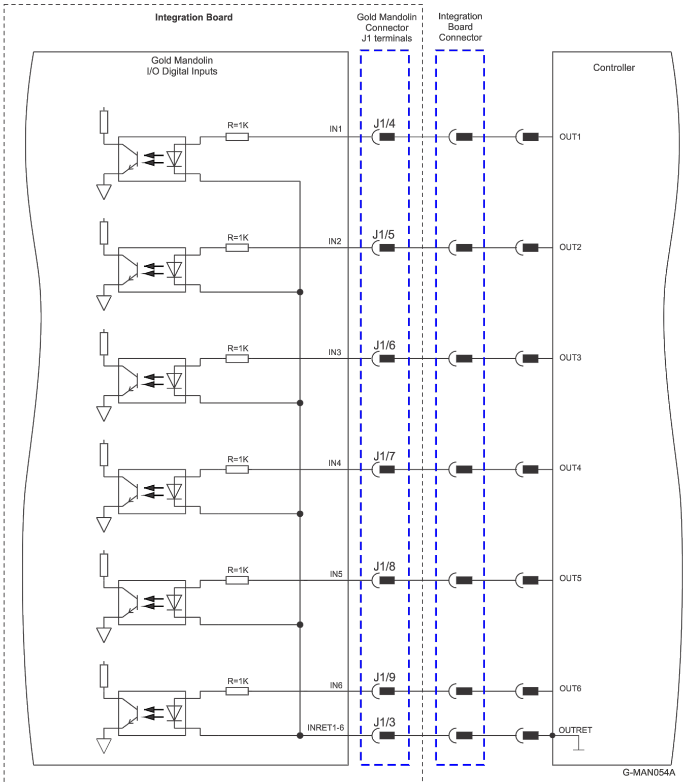
Figure 30: Digital Input TTL Mode Connection Diagram
