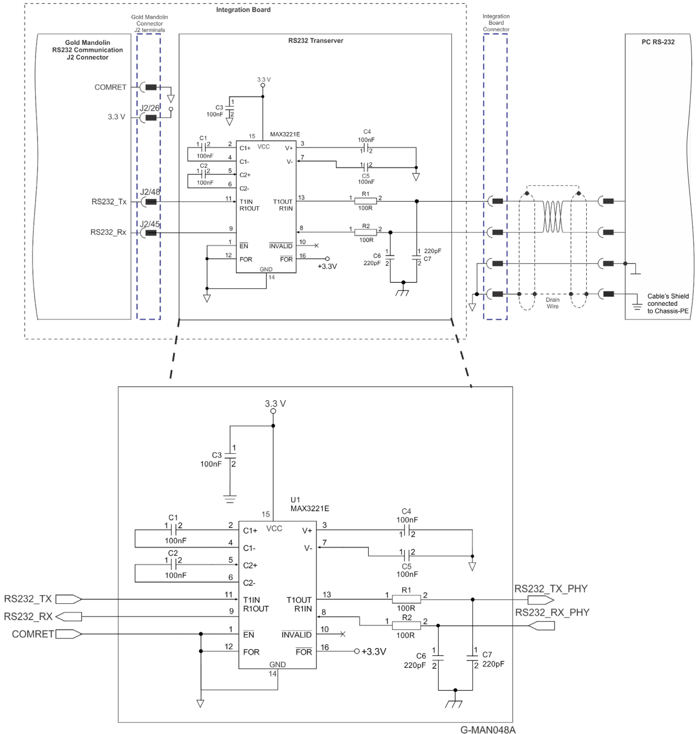
Figure 26: Standard RS232 Voltage Level incorporating RS232 TX/RX Transceiver Connection Diagram
