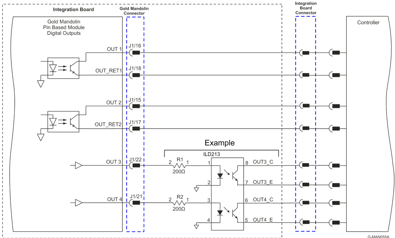
Figure 31: Digital Output Connection Diagram – Isolated Open Collector and Open Emitter Connection
