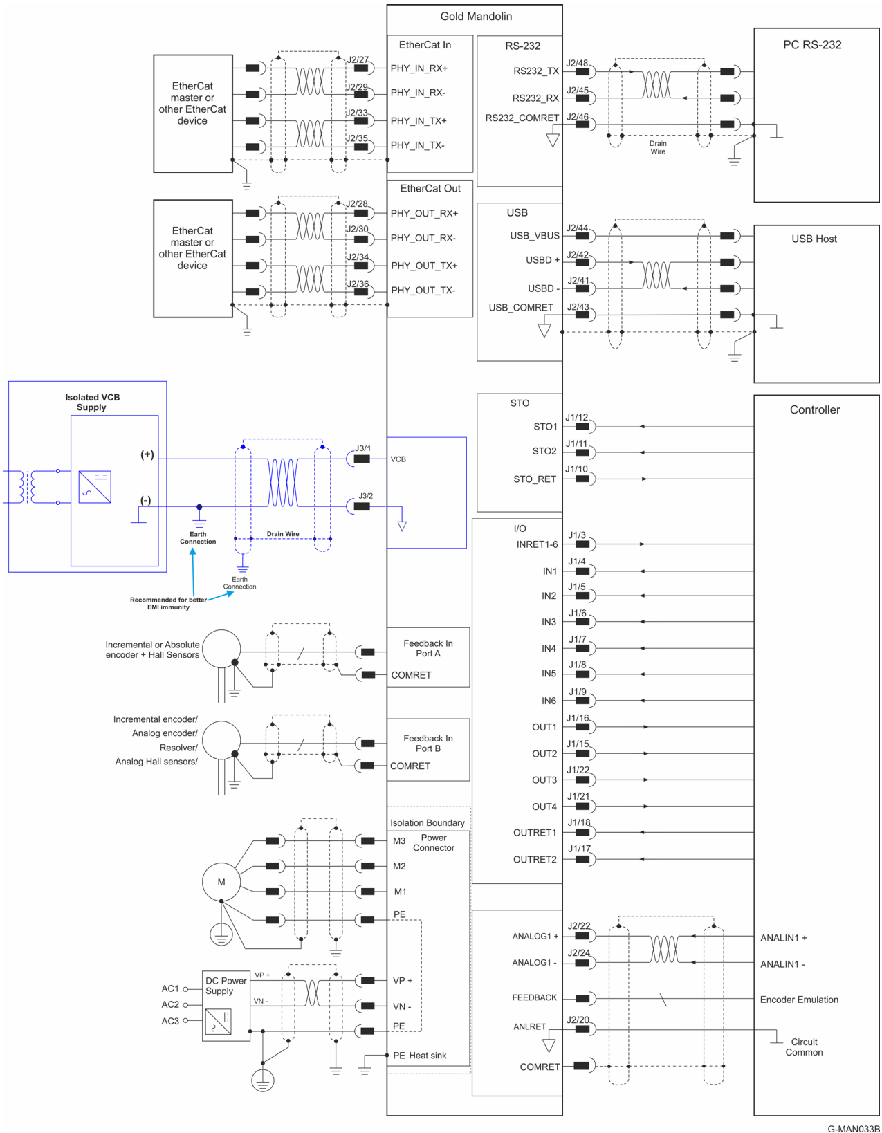
Figure 4: Gold Mandolin Connection Diagram for EtherCAT
