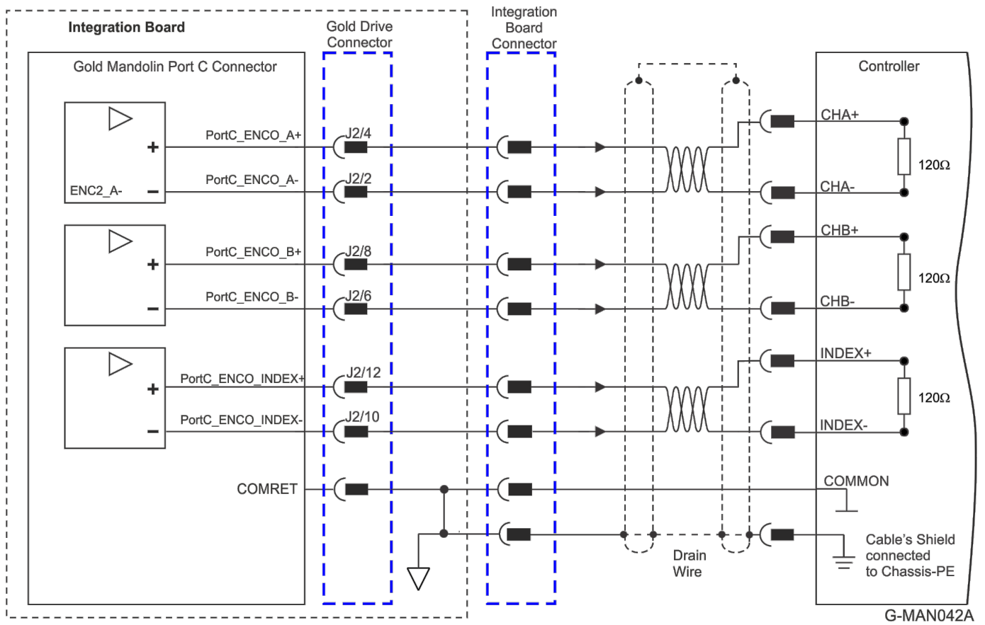
Figure 23: Emulated Encoder Differential Output – Recommended Connection Diagram
