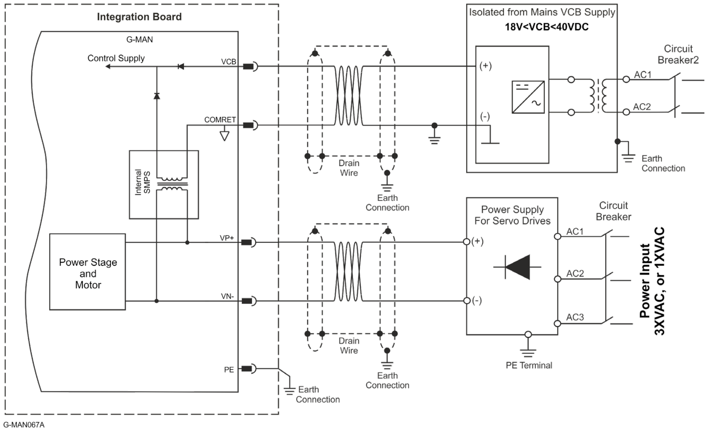
Figure 14: Gold Mandolin VP+ and VCB Topology
