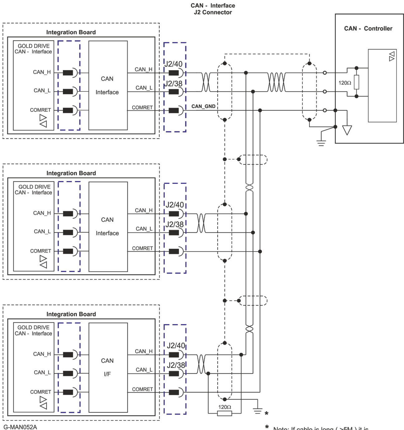
Figure 29: CANbus Connections
