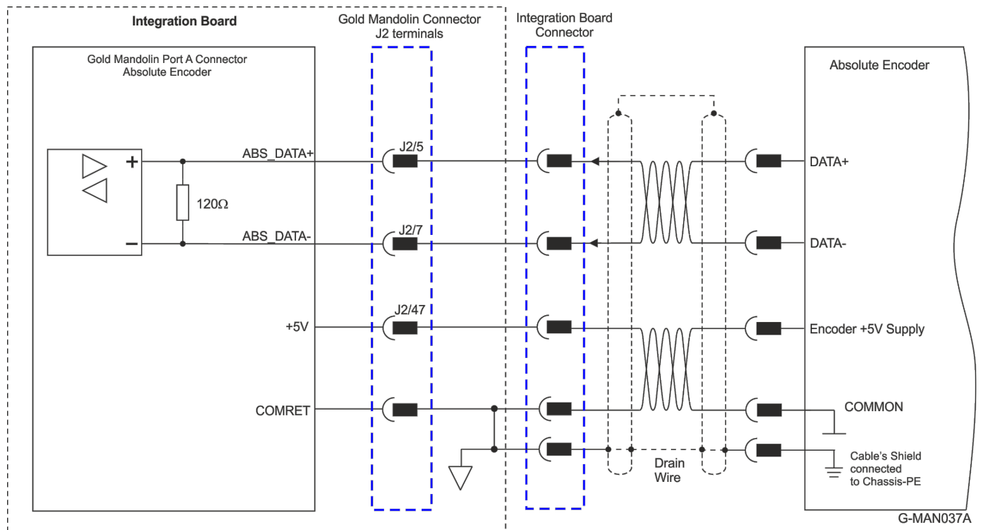
Figure 18: Absolute Serial Encoder – Recommended Connection Diagram for Panasonic, Tamgawai, Sanyo-Danki
