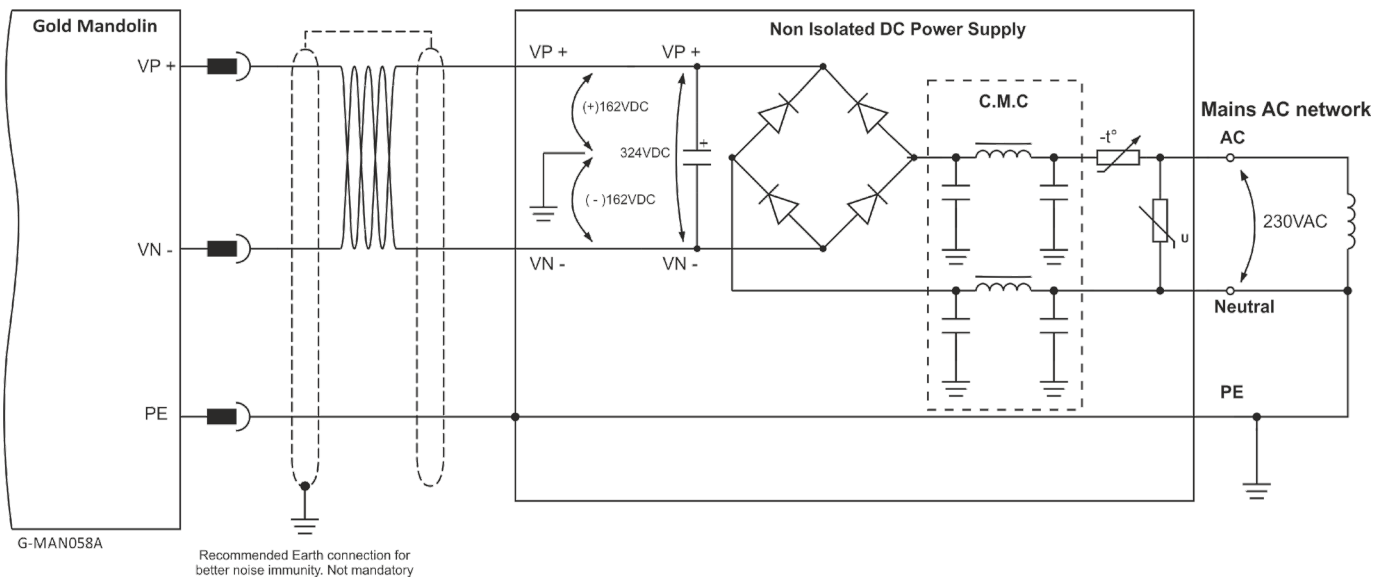
Figure 9: Non-Isolated Single-Phase Connection Topology
