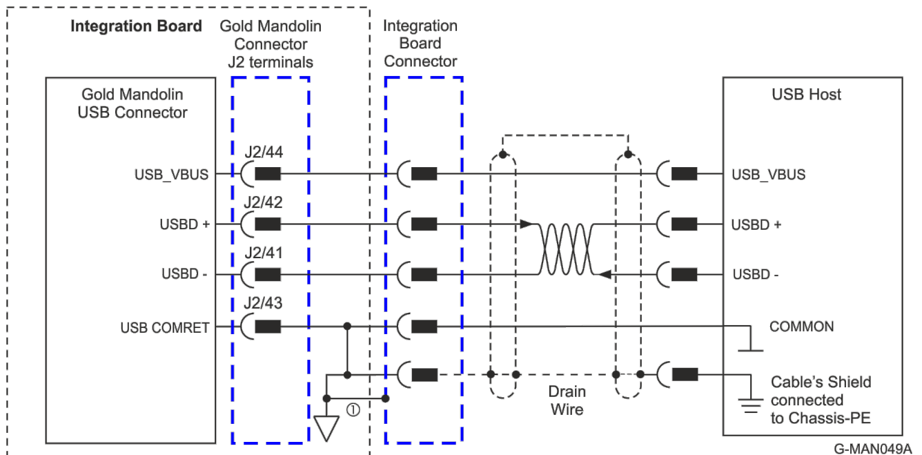
Figure 27: USB Network Diagram
