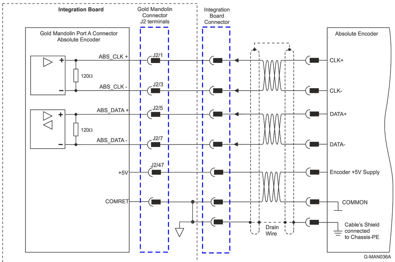
Figure 17: Absolute Serial Encoder – Recommended Connection Diagram for Endat, Biss, SSI
