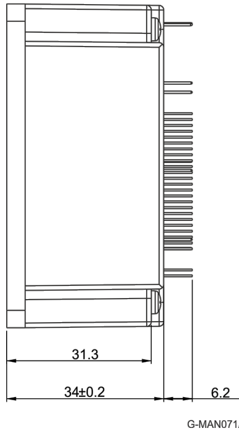
Figure 2: Gold Mandolin Footprint – Side
