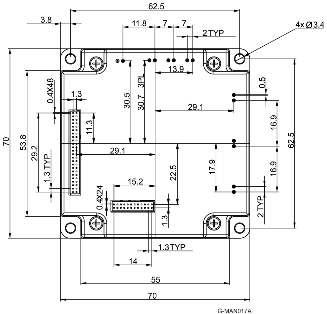
Figure 1: Gold Mandolin Footprint – Top
