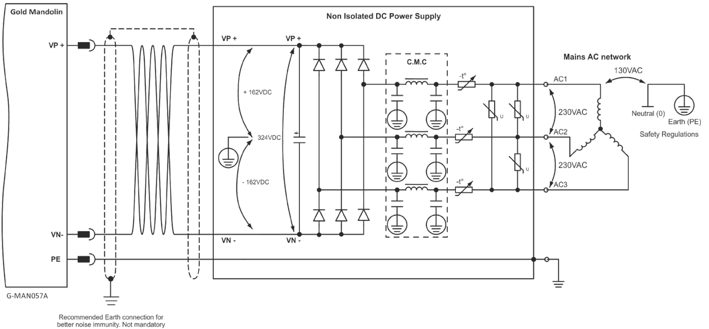
Figure 8: Non-Isolated Three-Phase Connection Topology
