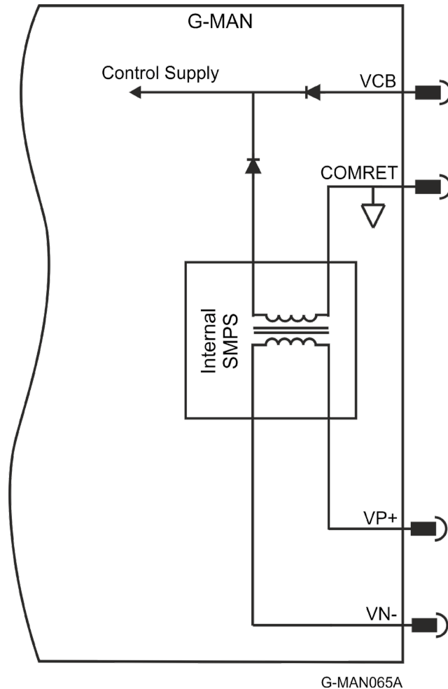
Figure 12: Switch-mode Power Supply
