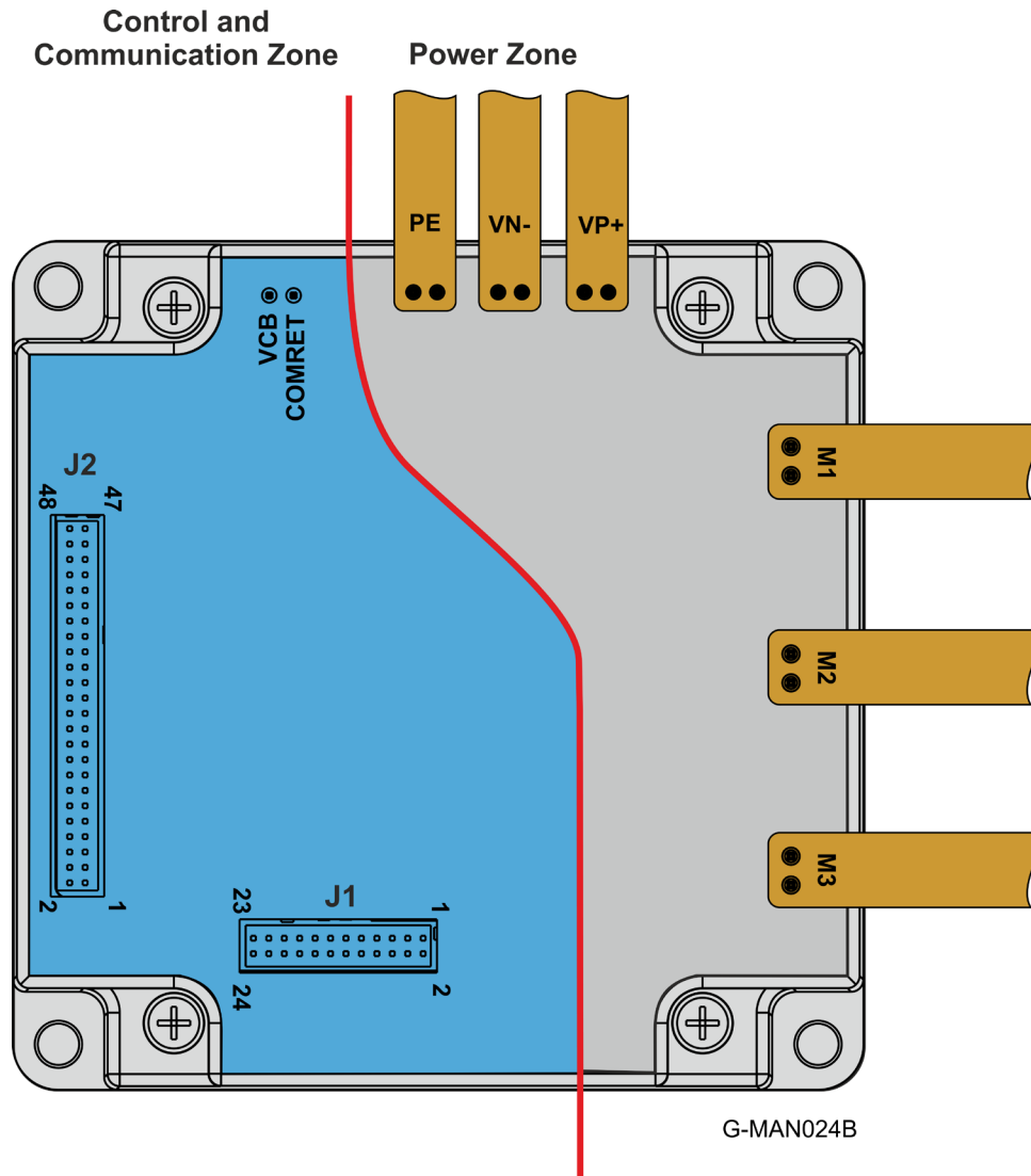
Figure 3: Gold Mandolin Power Conductors PCB layout
