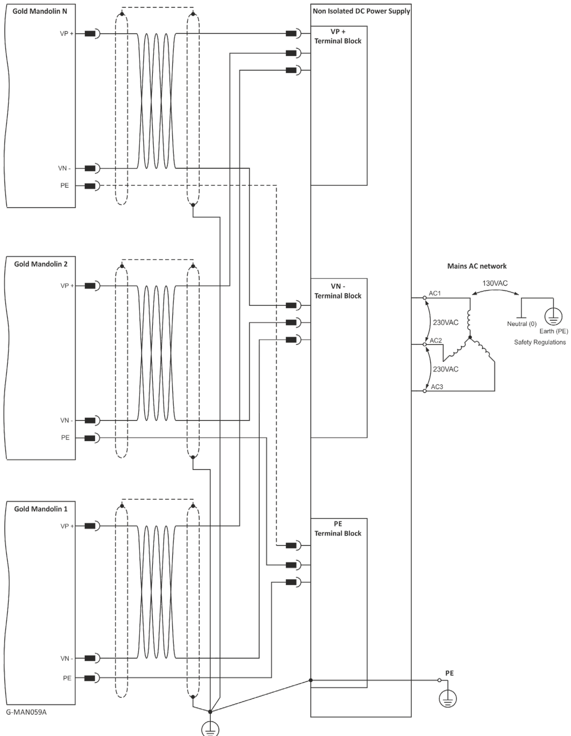
Figure 10: Non-Isolated Three-Phase Multiple Connection Topology
