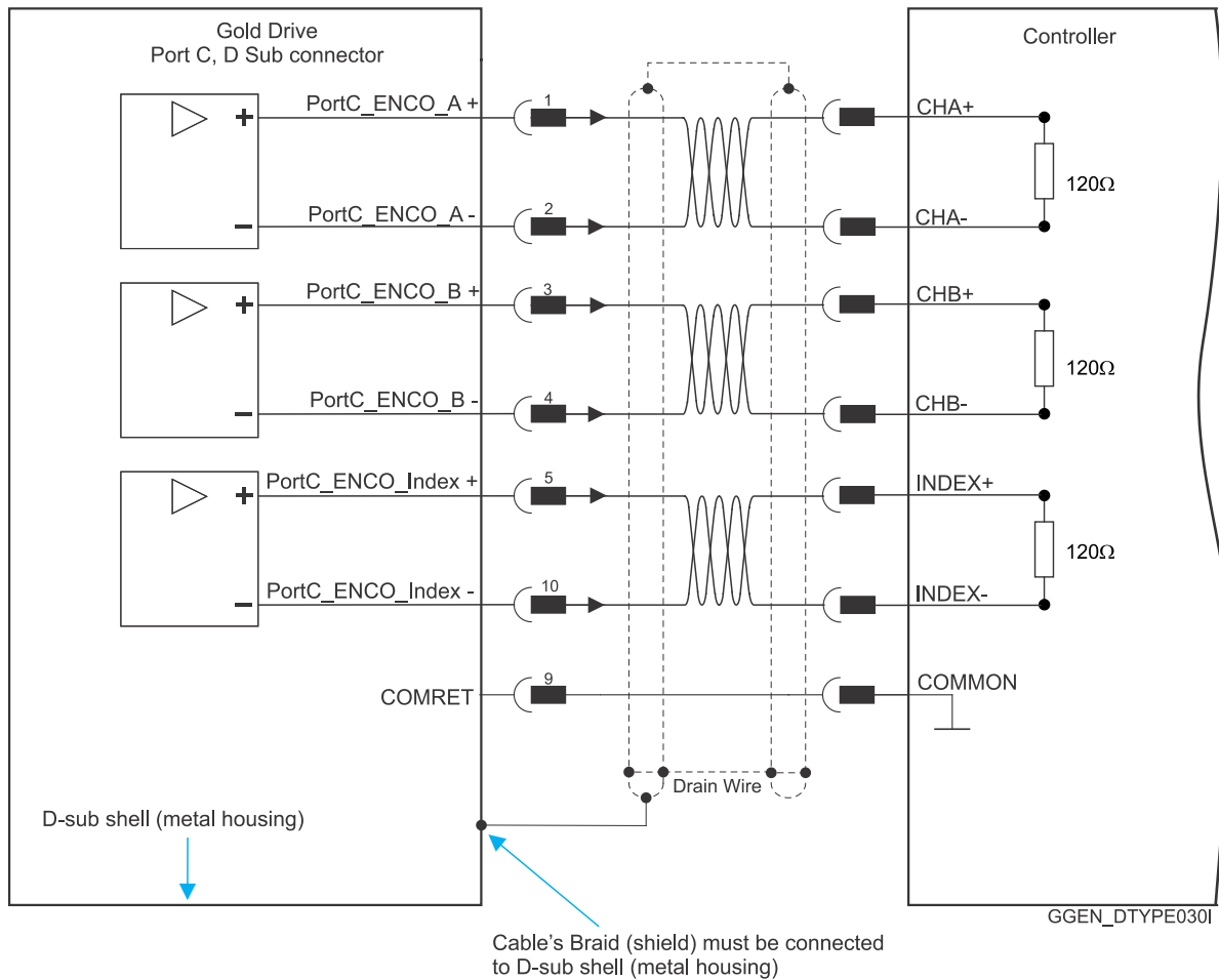
Figure 23: Encoder Differential Output – Recommended D-Type Connection Diagram
