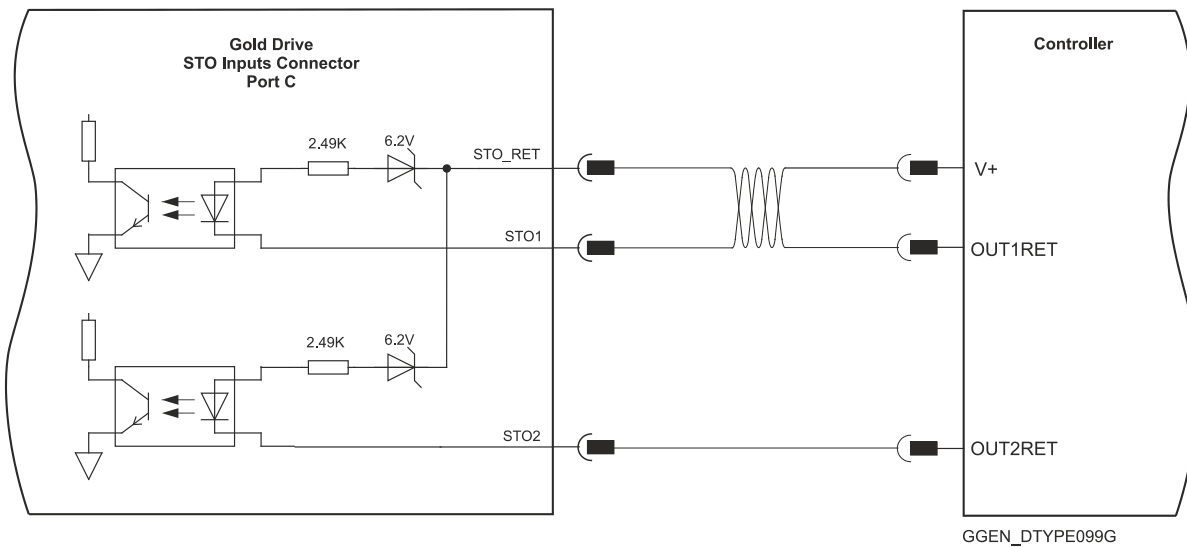
Figure 27: STO Input Connection – Sink Option
